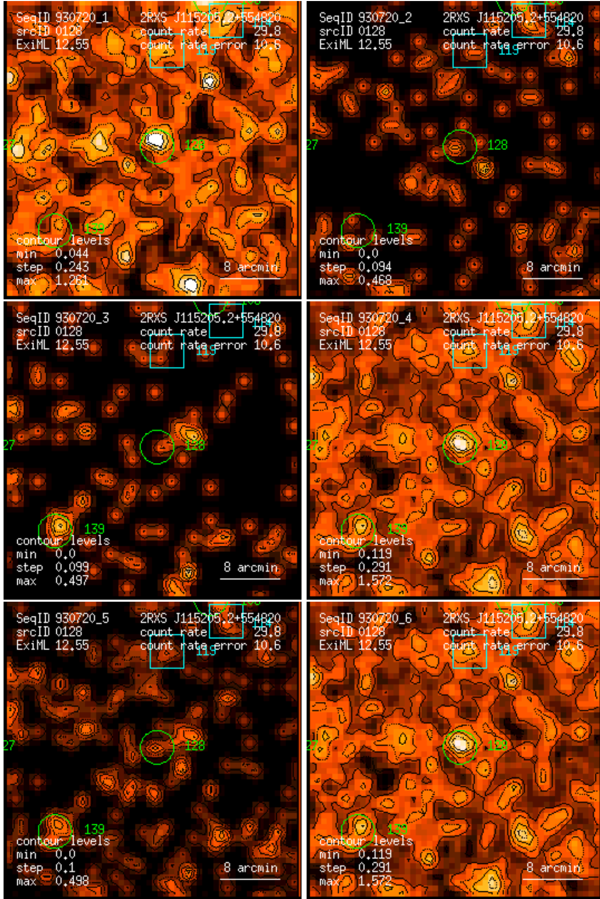
Figure 128: RASS 930720: detection 0128: band rate images, Gaussian filter: (1) PSPC channels 11 – 41, (2) 52 – 90, (3) 91 – 201, (4) 11 – 235, (5) 52 – 201, (6) 11 – 201. Broad band rates in counts/ks. Band rate contour levels in counts/ks/arcmin 2 .
