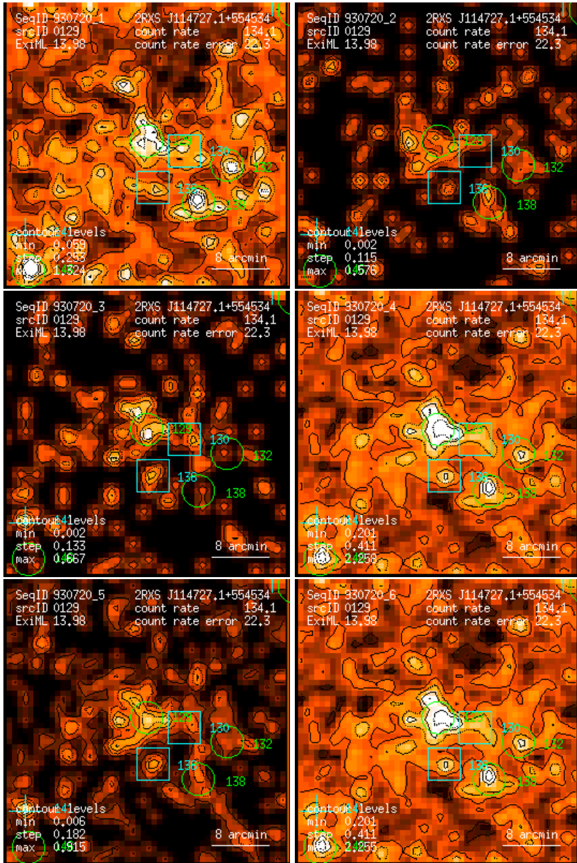
Figure 129: RASS 930720: detection 0129: band rate images, Gaussian filter: (1) PSPC channels 11 – 41, (2) 52 – 90, (3) 91 – 201, (4) 11 – 235, (5) 52 – 201, (6) 11 – 201. Broad band rates in counts/ks. Band rate contour levels in counts/ks/arcmin 2 .
