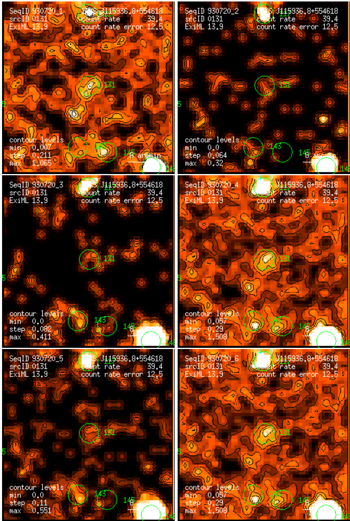
Figure 131: RASS 930720: detection 0131: band rate images, Gaussian filter: (1) PSPC channels 11 – 41, (2) 52 – 90, (3) 91 – 201, (4) 11 – 235, (5) 52 – 201, (6) 11 – 201. Broad band rates in counts/ks. Band rate contour levels in counts/ks/arcmin 2 .
