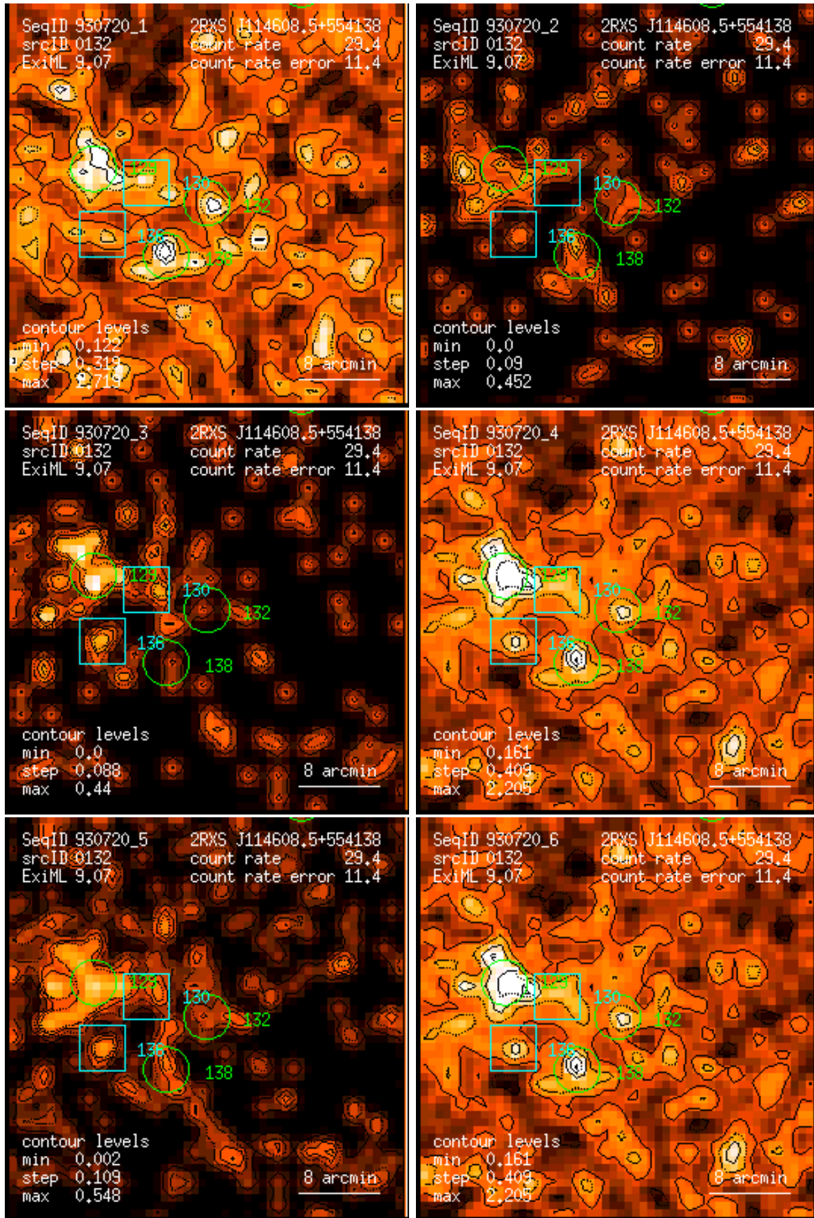
Figure 132: RASS 930720: detection 0132: band rate images, Gaussian filter: (1) PSPC channels 11 – 41, (2) 52 – 90, (3) 91 – 201, (4) 11 – 235, (5) 52 – 201, (6) 11 – 201. Broad band rates in counts/ks. Band rate contour levels in counts/ks/arcmin 2 .
