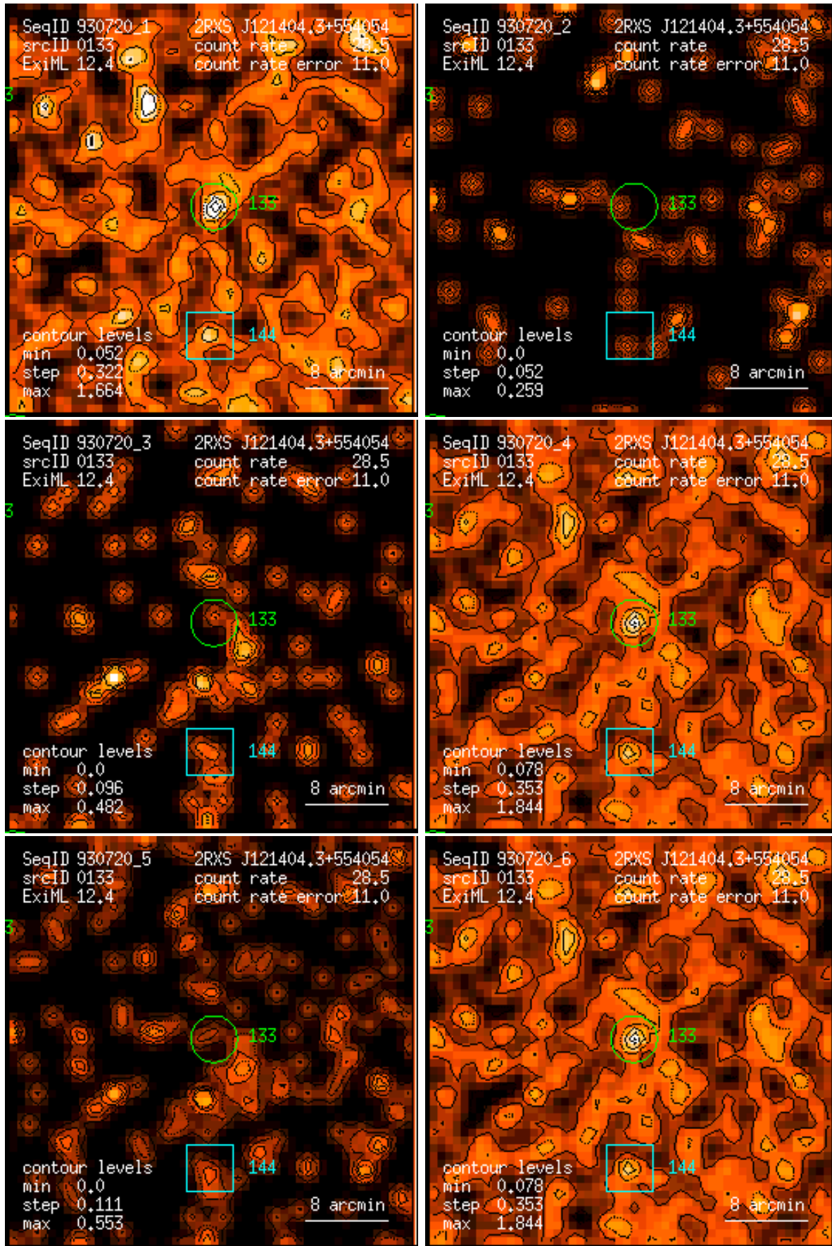
Figure 133: RASS 930720: detection 0133: band rate images, Gaussian filter: (1) PSPC channels 11 – 41, (2) 52 – 90, (3) 91 – 201, (4) 11 – 235, (5) 52 – 201, (6) 11 – 201. Broad band rates in counts/ks. Band rate contour levels in counts/ks/arcmin 2 .
