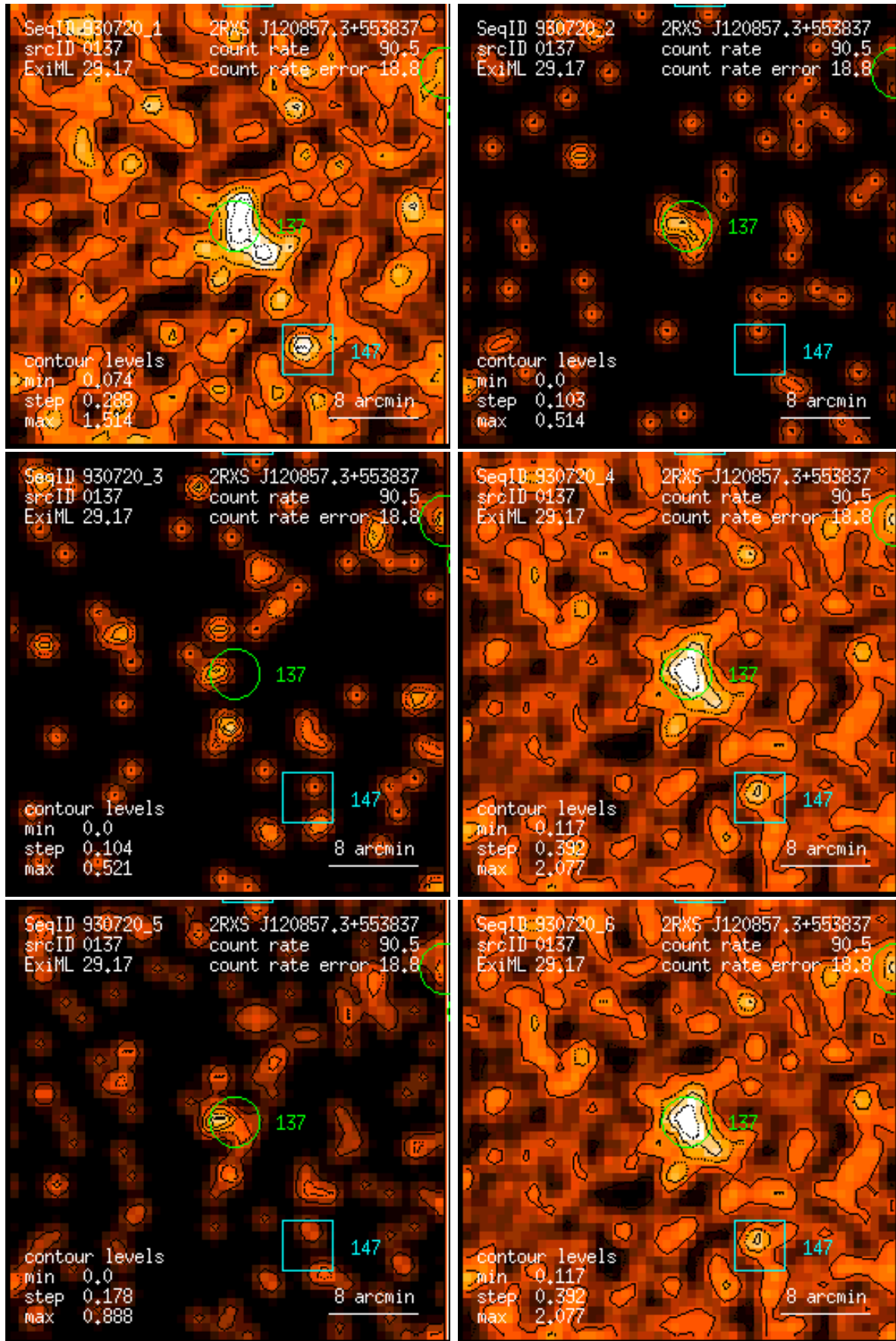
Figure 137: RASS 930720: detection 0137: band rate images, Gaussian filter: (1) PSPC channels 11 – 41, (2) 52 – 90, (3) 91 – 201, (4) 11 – 235, (5) 52 – 201, (6) 11 – 201. Broad band rates in counts/ks. Band rate contour levels in counts/ks/arcmin 2 .
