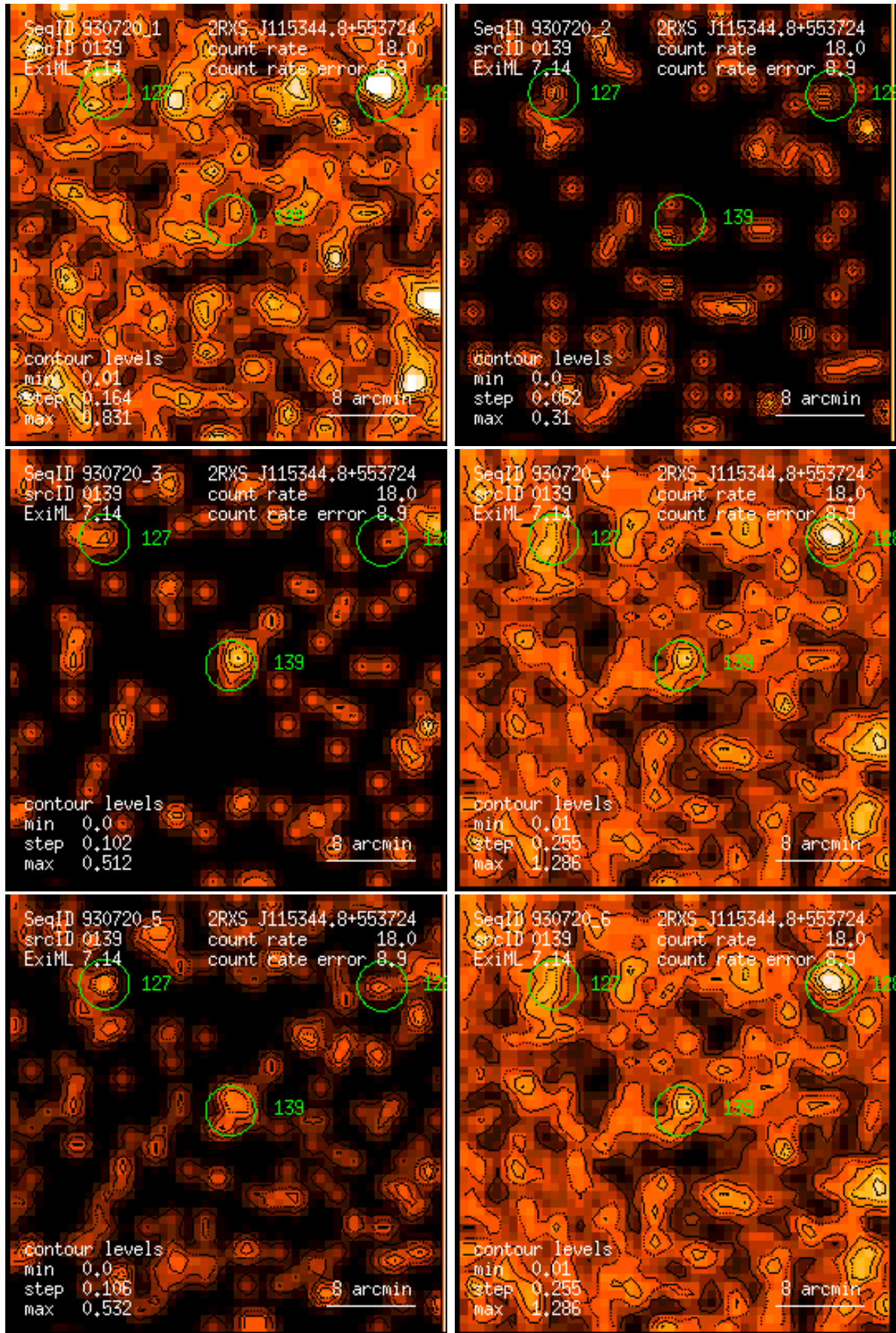
Figure 139: RASS 930720: detection 0139: band rate images, Gaussian filter: (1) PSPC channels 11 – 41, (2) 52 – 90, (3) 91 – 201, (4) 11 – 235, (5) 52 – 201, (6) 11 – 201. Broad band rates in counts/ks. Band rate contour levels in counts/ks/arcmin 2 .
