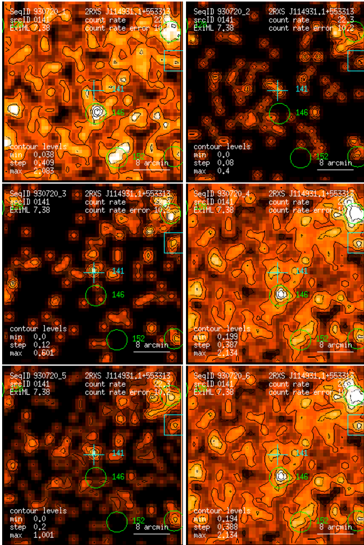
Figure 141: RASS 930720: detection 0141: band rate images, Gaussian filter: (1) PSPC channels 11 – 41, (2) 52 – 90, (3) 91 – 201, (4) 11 – 235, (5) 52 – 201, (6) 11 – 201. Broad band rates in counts/ks. Band rate contour levels in counts/ks/arcmin 2 .
