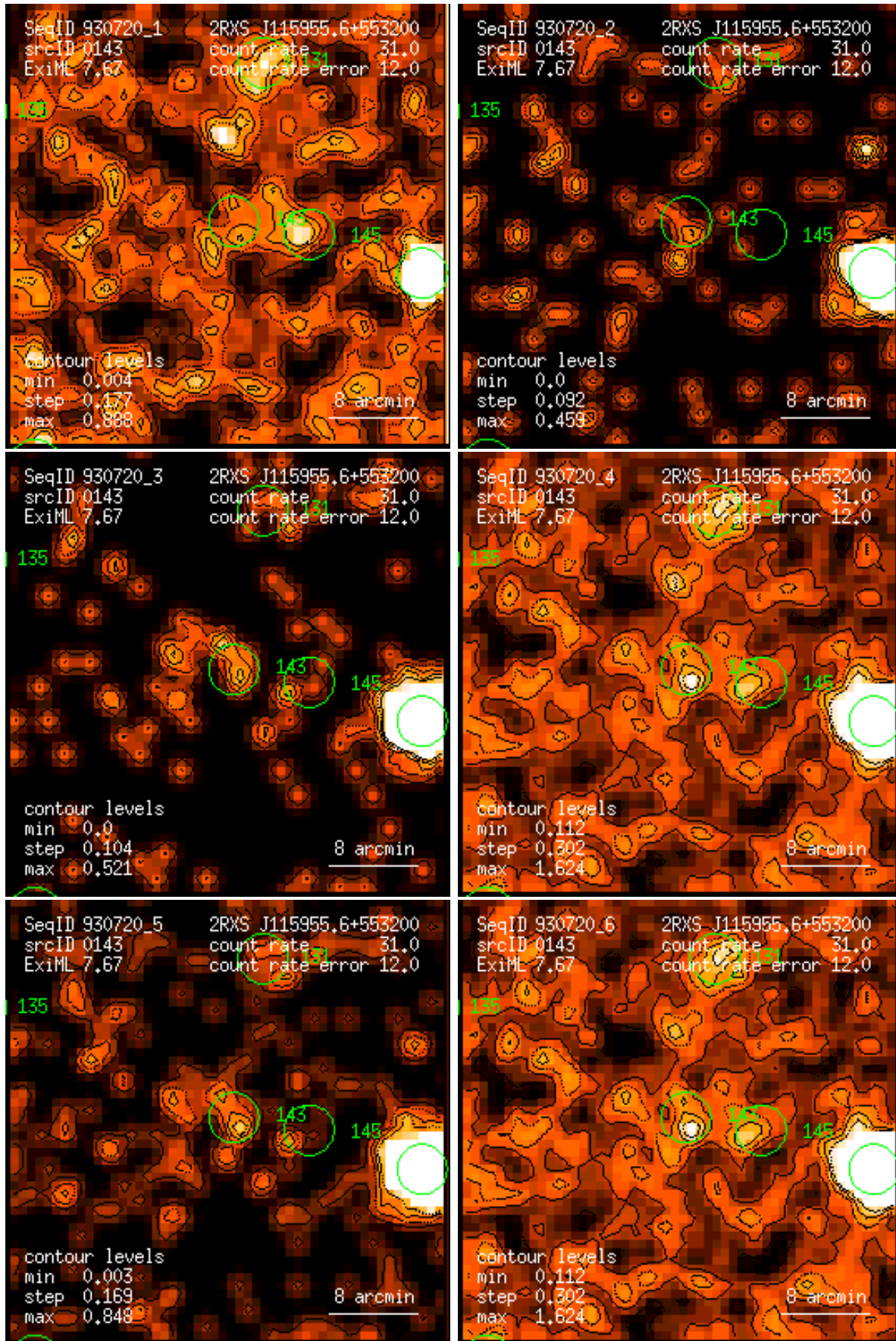
Figure 143: RASS 930720: detection 0143: band rate images, Gaussian filter: (1) PSPC channels 11 – 41, (2) 52 – 90, (3) 91 – 201, (4) 11 – 235, (5) 52 – 201, (6) 11 – 201. Broad band rates in counts/ks. Band rate contour levels in counts/ks/arcmin 2 .
