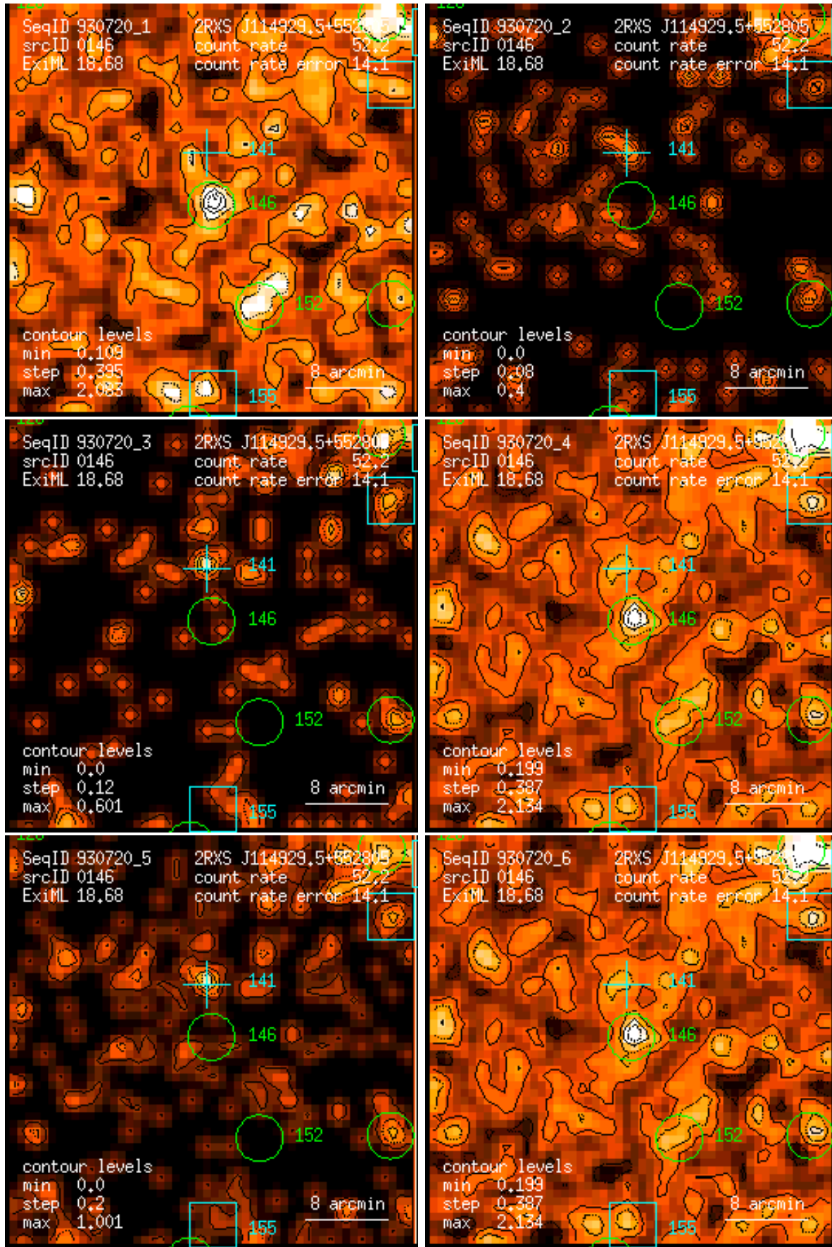
Figure 146: RASS 930720: detection 0146: band rate images, Gaussian filter: (1) PSPC channels 11 – 41, (2) 52 – 90, (3) 91 – 201, (4) 11 – 235, (5) 52 – 201, (6) 11 – 201. Broad band rates in counts/ks. Band rate contour levels in counts/ks/arcmin 2 .
