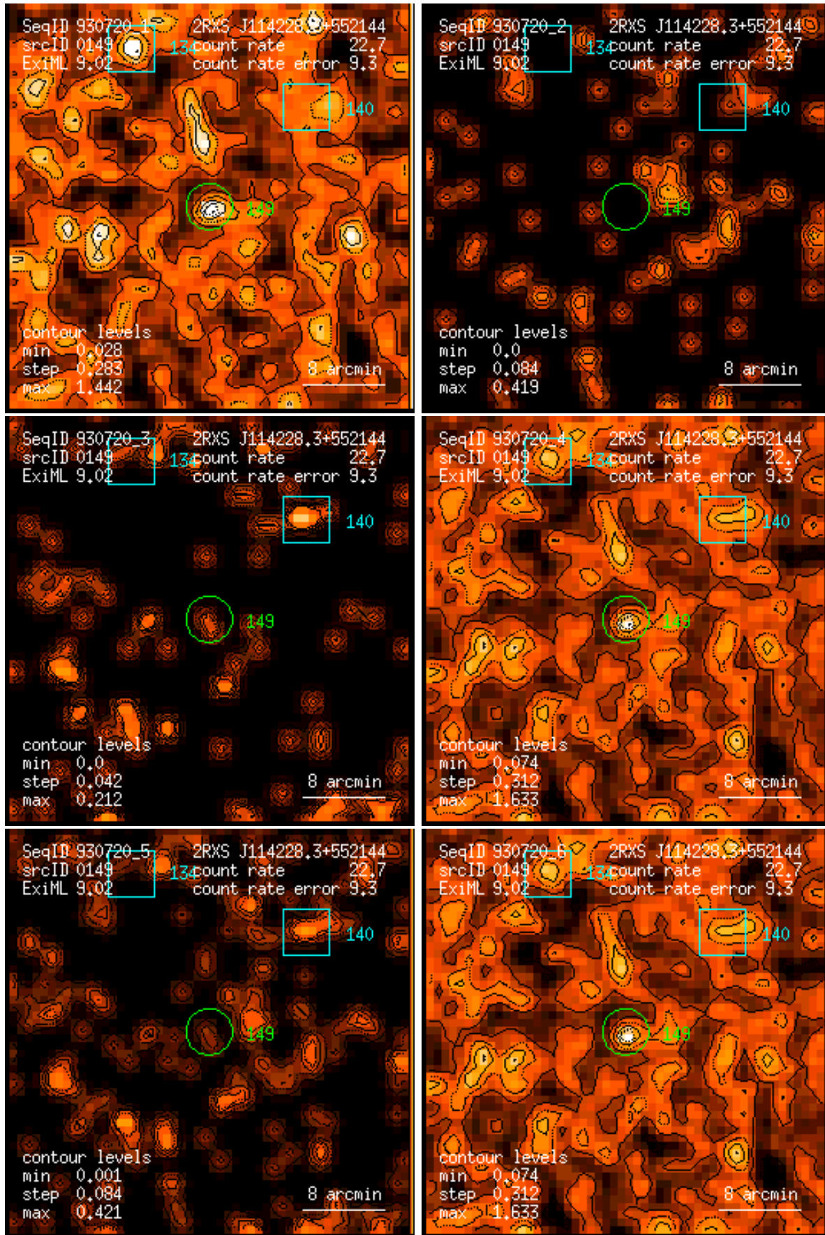
Figure 149: RASS 930720: detection 0149: band rate images, Gaussian filter: (1) PSPC channels 11 – 41, (2) 52 – 90, (3) 91 – 201, (4) 11 – 235, (5) 52 – 201, (6) 11 – 201. Broad band rates in counts/ks. Band rate contour levels in counts/ks/arcmin 2 .
