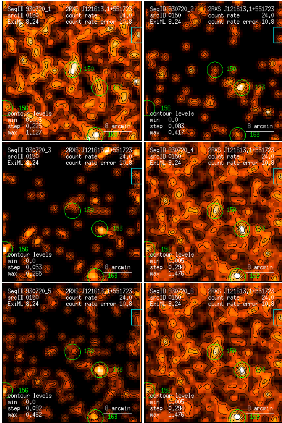
Figure 150: RASS 930720: detection 0150: band rate images, Gaussian filter: (1) PSPC channels 11 – 41, (2) 52 – 90, (3) 91 – 201, (4) 11 – 235, (5) 52 – 201, (6) 11 – 201. Broad band rates in counts/ks. Band rate contour levels in counts/ks/arcmin 2 .
