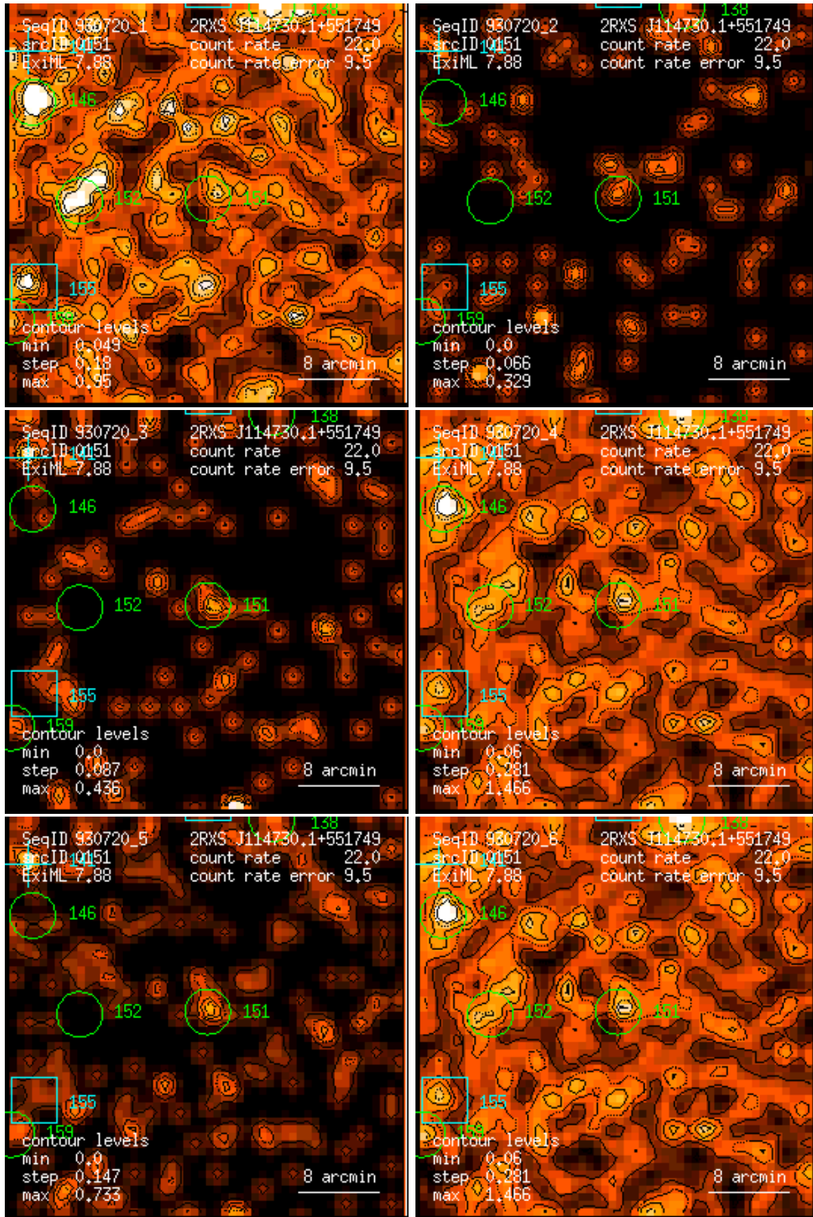
Figure 151: RASS 930720: detection 0151: band rate images, Gaussian filter: (1) PSPC channels 11 – 41, (2) 52 – 90, (3) 91 – 201, (4) 11 – 235, (5) 52 – 201, (6) 11 – 201. Broad band rates in counts/ks. Band rate contour levels in counts/ks/arcmin 2 .
