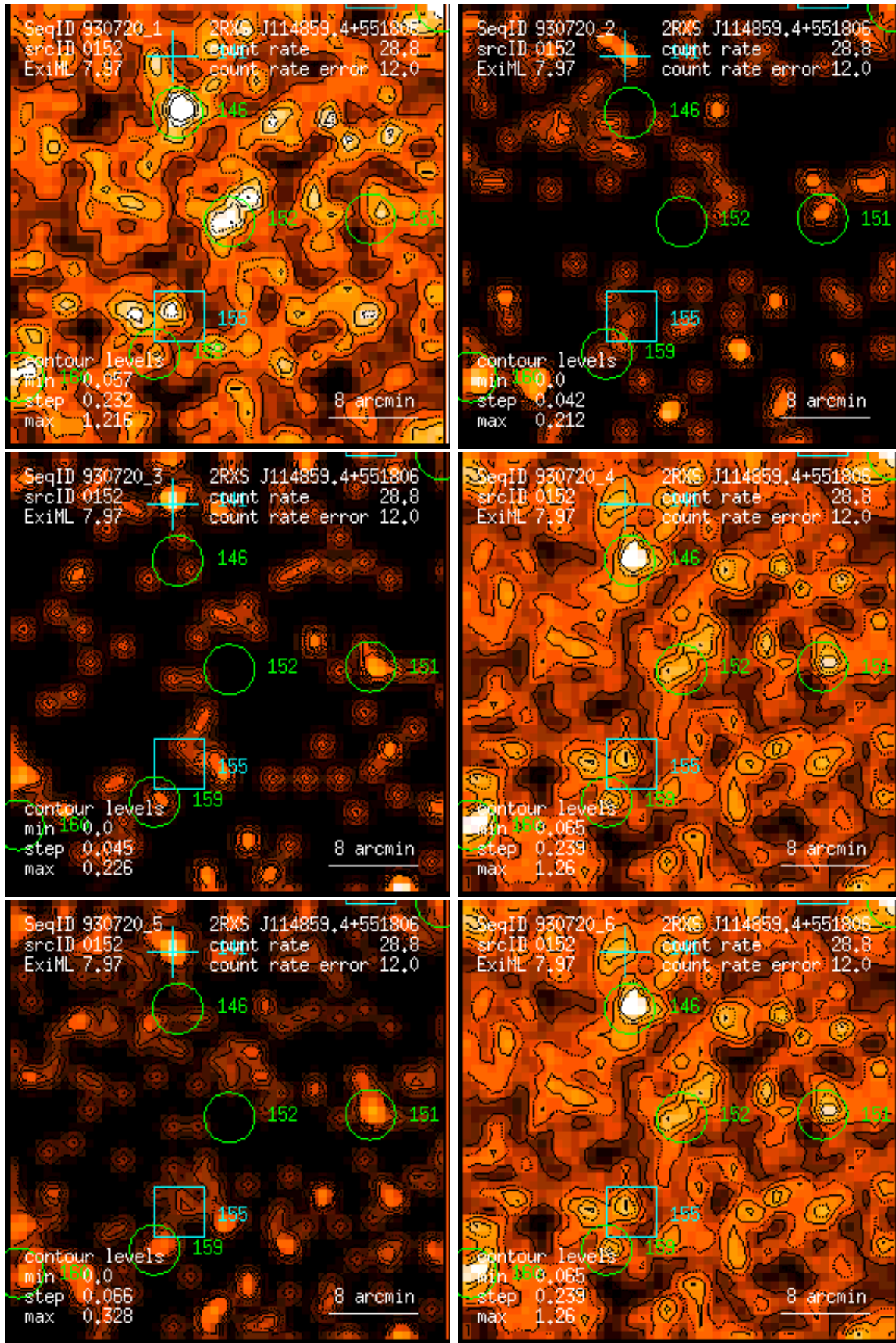
Figure 152: RASS 930720: detection 0152: band rate images, Gaussian filter: (1) PSPC channels 11 – 41, (2) 52 – 90, (3) 91 – 201, (4) 11 – 235, (5) 52 – 201, (6) 11 – 201. Broad band rates in counts/ks. Band rate contour levels in counts/ks/arcmin 2 .
