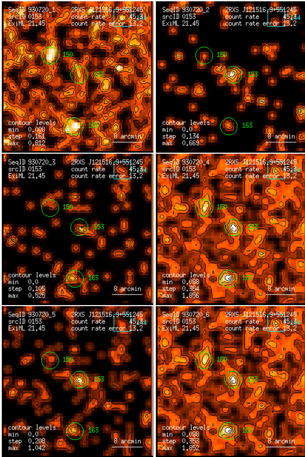
Figure 153: RASS 930720: detection 0153: band rate images, Gaussian filter: (1) PSPC channels 11 – 41, (2) 52 – 90, (3) 91 – 201, (4) 11 – 235, (5) 52 – 201, (6) 11 – 201. Broad band rates in counts/ks. Band rate contour levels in counts/ks/arcmin 2 .
