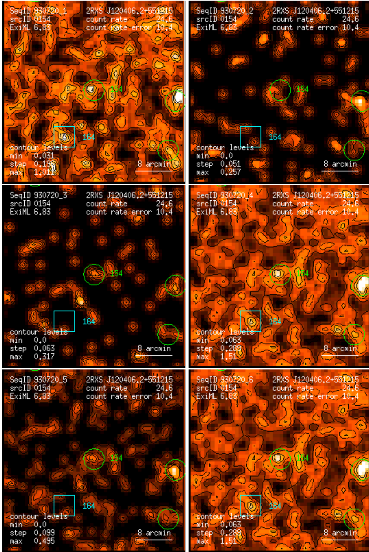
Figure 154: RASS 930720: detection 0154: band rate images, Gaussian filter: (1) PSPC channels 11 – 41, (2) 52 – 90, (3) 91 – 201, (4) 11 – 235, (5) 52 – 201, (6) 11 – 201. Broad band rates in counts/ks. Band rate contour levels in counts/ks/arcmin 2 .
