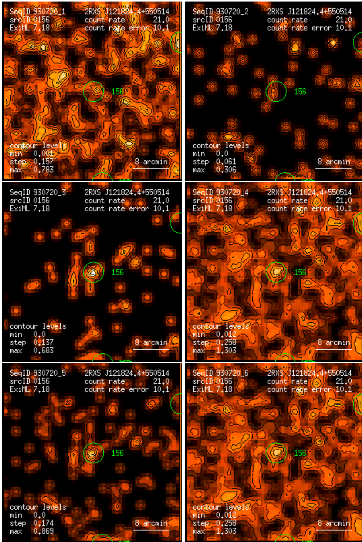
Figure 156: RASS 930720: detection 0156: band rate images, Gaussian filter: (1) PSPC channels 11 – 41, (2) 52 – 90, (3) 91 – 201, (4) 11 – 235, (5) 52 – 201, (6) 11 – 201. Broad band rates in counts/ks. Band rate contour levels in counts/ks/arcmin 2 .
