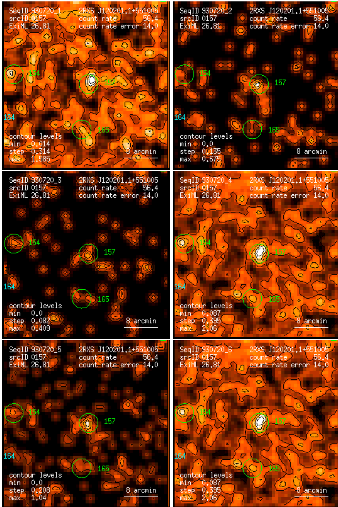
Figure 157: RASS 930720: detection 0157: band rate images, Gaussian filter: (1) PSPC channels 11 – 41, (2) 52 – 90, (3) 91 – 201, (4) 11 – 235, (5) 52 – 201, (6) 11 – 201. Broad band rates in counts/ks. Band rate contour levels in counts/ks/arcmin 2 .
