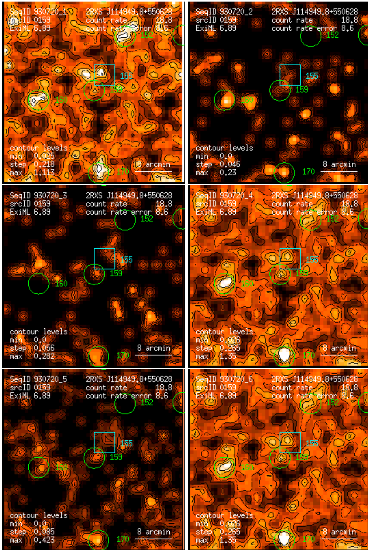
Figure 159: RASS 930720: detection 0159: band rate images, Gaussian filter: (1) PSPC channels 11 – 41, (2) 52 – 90, (3) 91 – 201, (4) 11 – 235, (5) 52 – 201, (6) 11 – 201. Broad band rates in counts/ks. Band rate contour levels in counts/ks/arcmin 2 .
