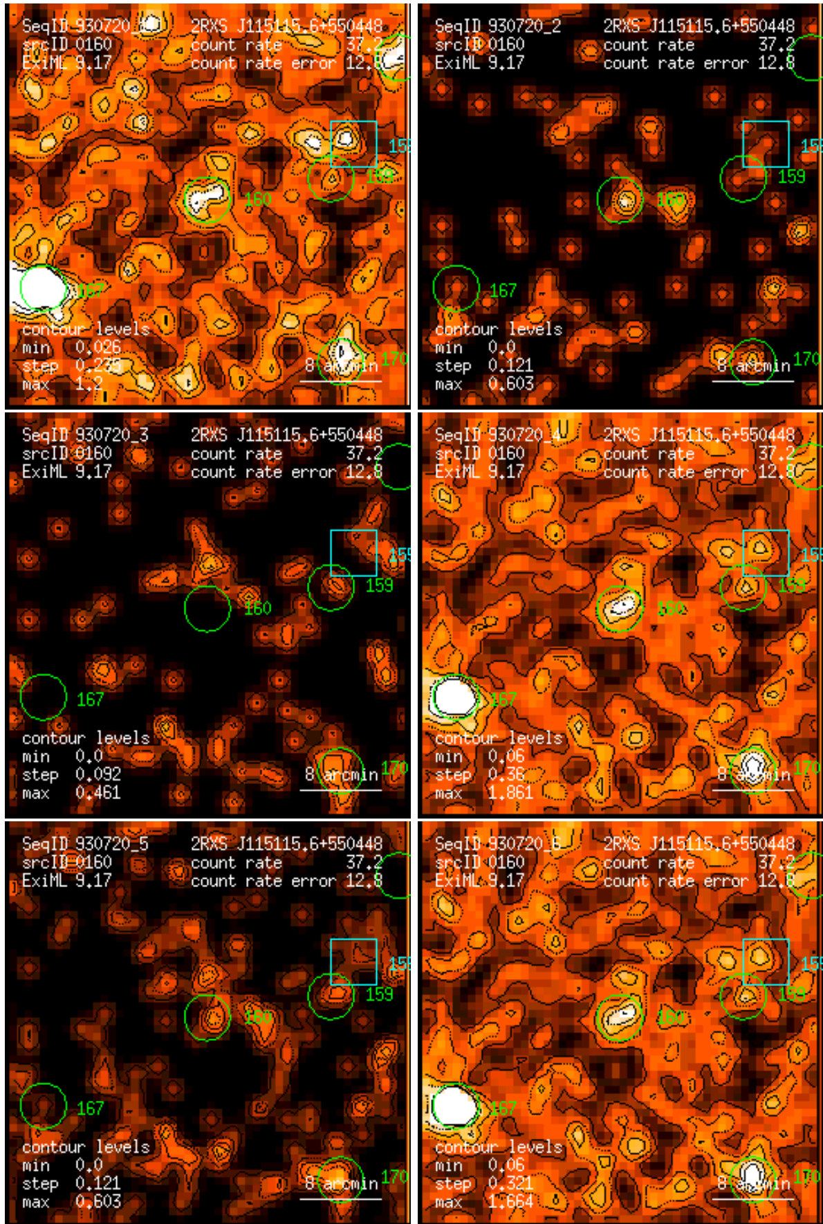
Figure 160: RASS 930720: detection 0160: band rate images, Gaussian filter: (1) PSPC channels 11 – 41, (2) 52 – 90, (3) 91 – 201, (4) 11 – 235, (5) 52 – 201, (6) 11 – 201. Broad band rates in counts/ks. Band rate contour levels in counts/ks/arcmin 2 .
