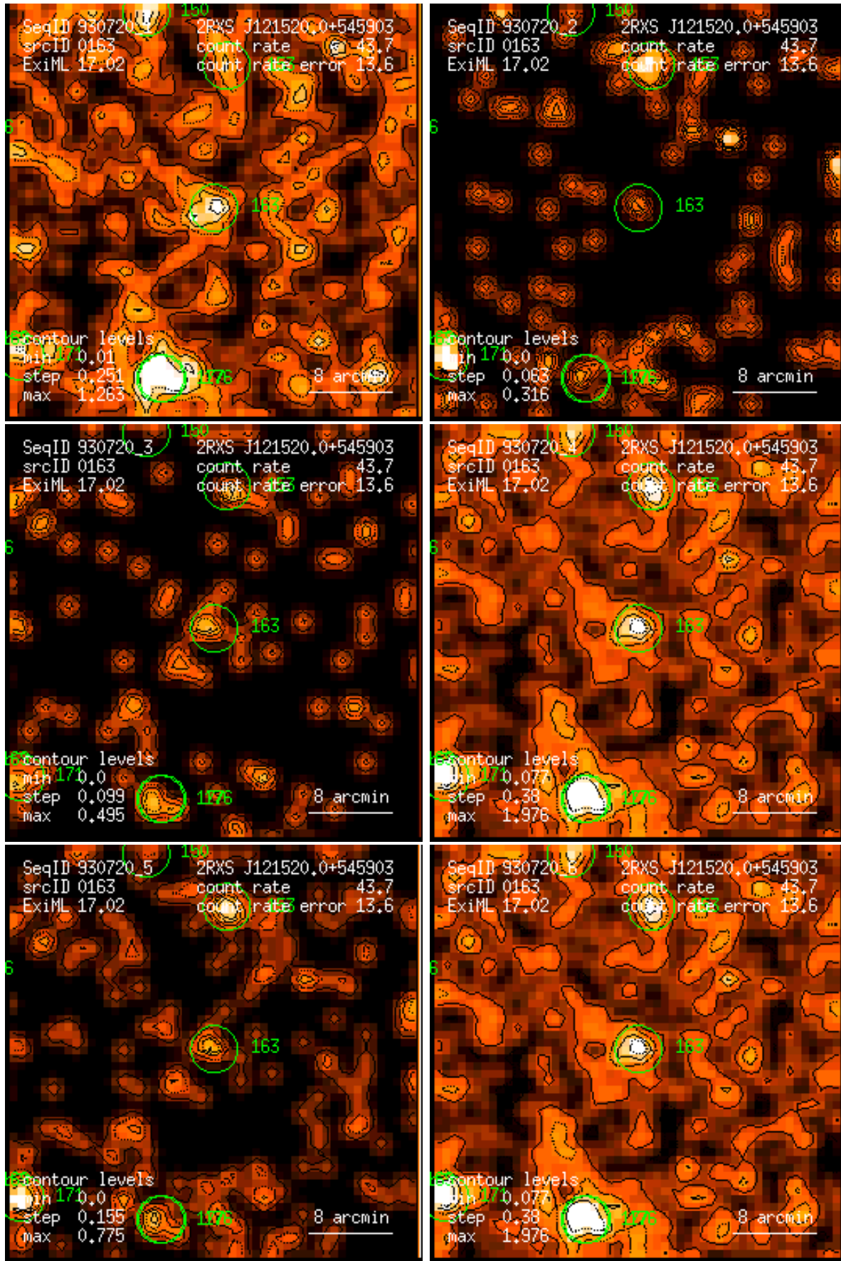
Figure 163: RASS 930720: detection 0163: band rate images, Gaussian filter: (1) PSPC channels 11 – 41, (2) 52 – 90, (3) 91 – 201, (4) 11 – 235, (5) 52 – 201, (6) 11 – 201. Broad band rates in counts/ks. Band rate contour levels in counts/ks/arcmin 2 .
