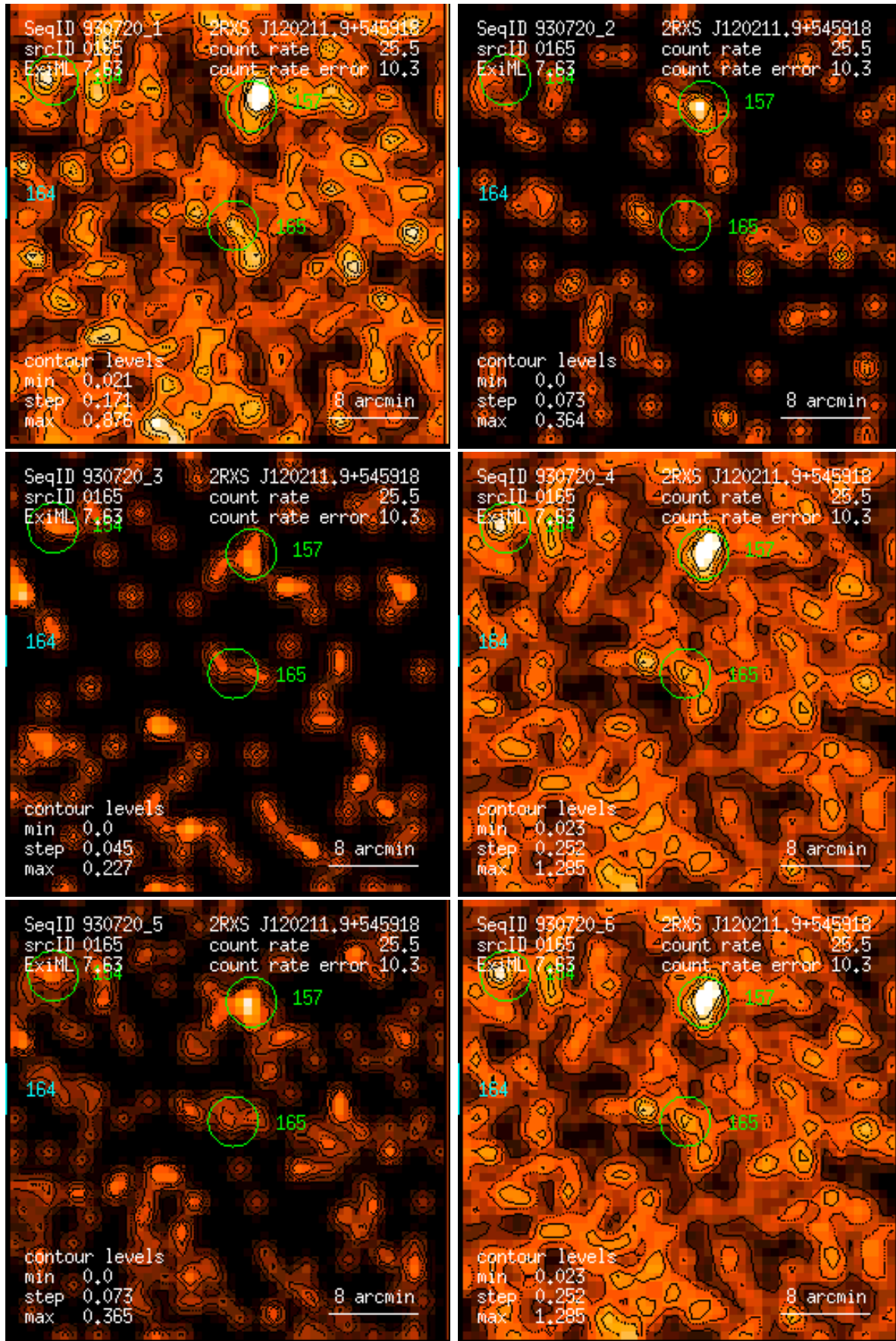
Figure 165: RASS 930720: detection 0165: band rate images, Gaussian filter: (1) PSPC channels 11 – 41, (2) 52 – 90, (3) 91 – 201, (4) 11 – 235, (5) 52 – 201, (6) 11 – 201. Broad band rates in counts/ks. Band rate contour levels in counts/ks/arcmin 2 .
