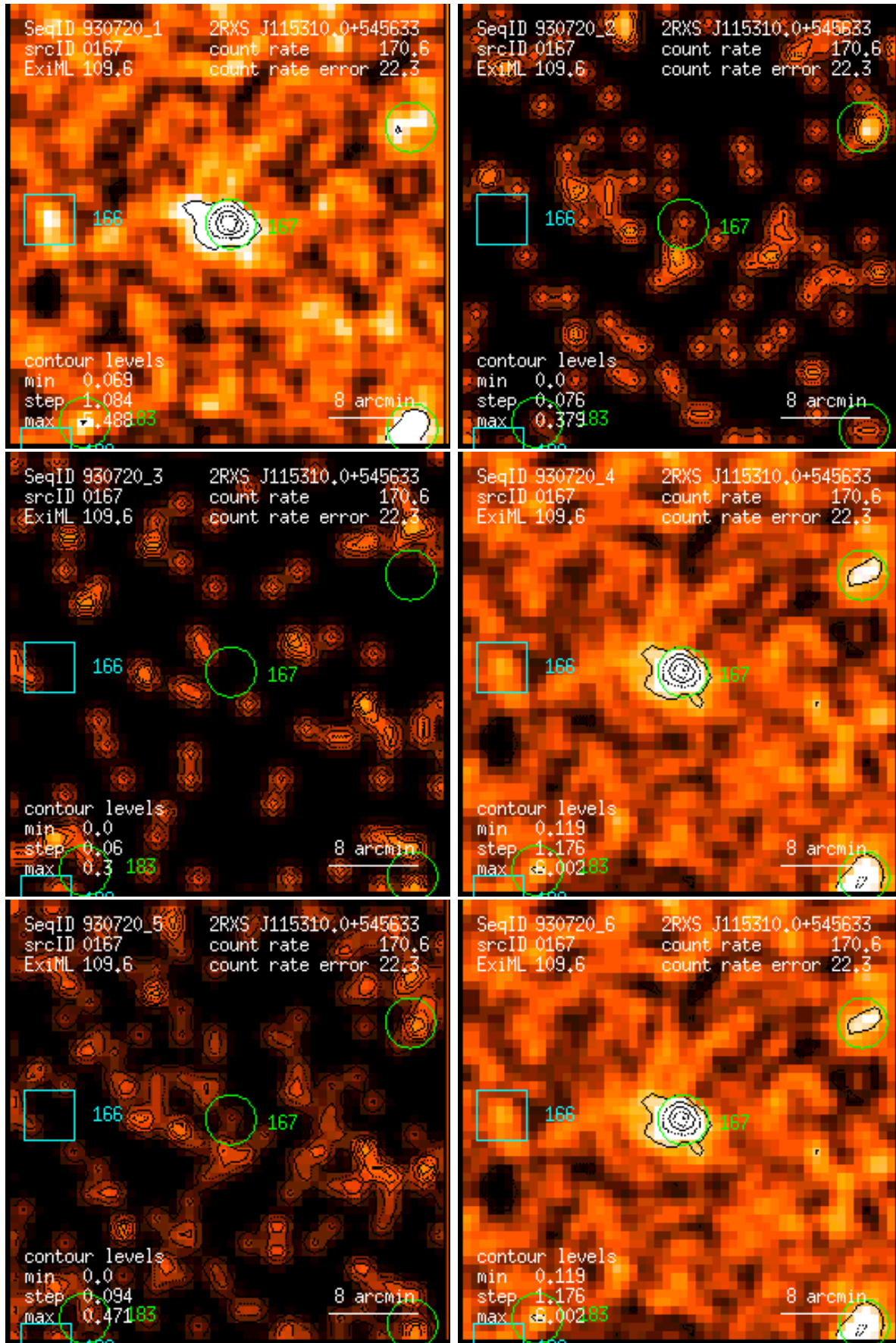
Figure 167: RASS 930720: detection 0167: band rate images, Gaussian filter: (1) PSPC channels 11 – 41, (2) 52 – 90, (3) 91 – 201, (4) 11 – 235, (5) 52 – 201, (6) 11 – 201. Broad band rates in counts/ks. Band rate contour levels in counts/ks/arcmin 2 .
