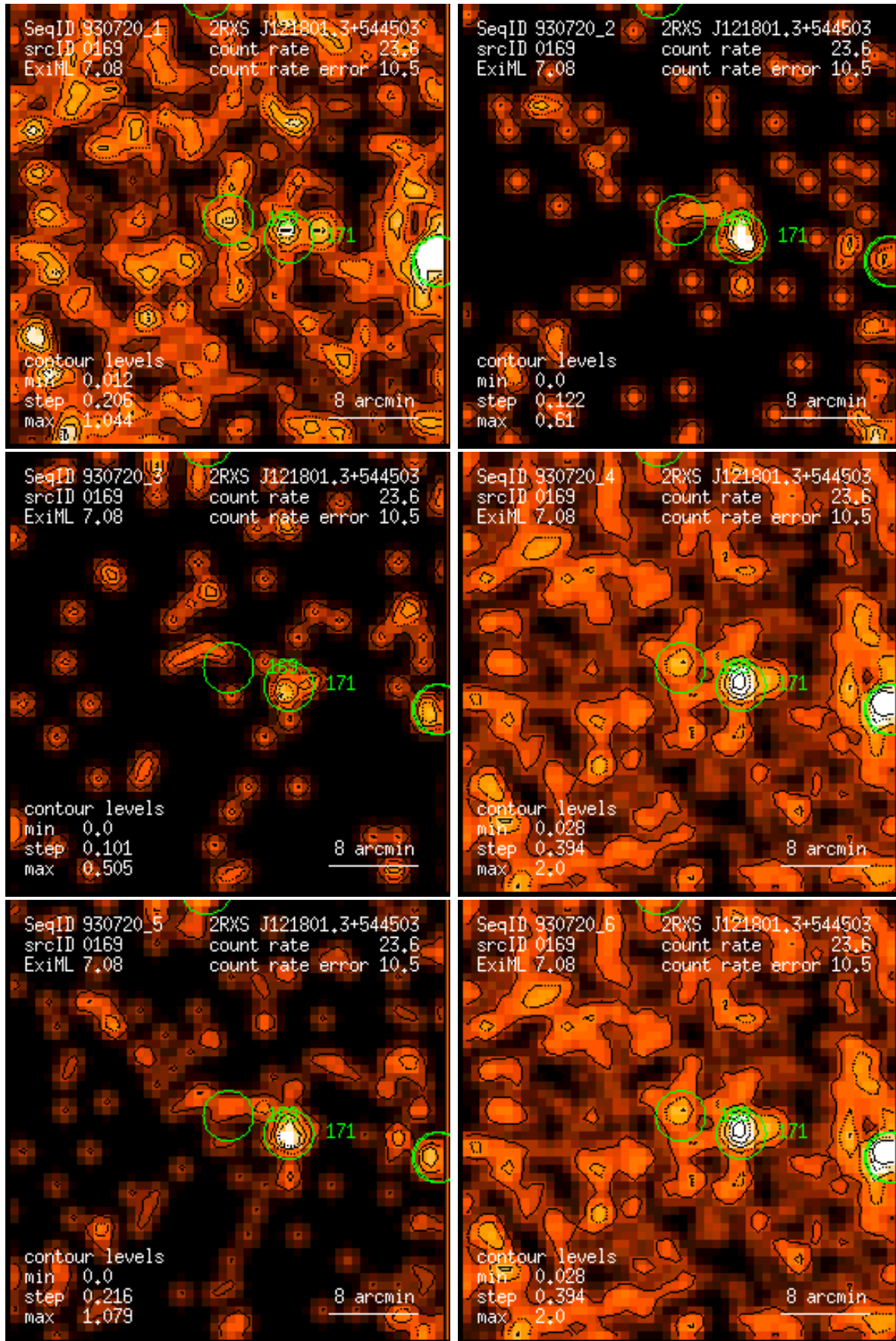
Figure 169: RASS 930720: detection 0169: band rate images, Gaussian filter: (1) PSPC channels 11 – 41, (2) 52 – 90, (3) 91 – 201, (4) 11 – 235, (5) 52 – 201, (6) 11 – 201. Broad band rates in counts/ks. Band rate contour levels in counts/ks/arcmin 2 .
