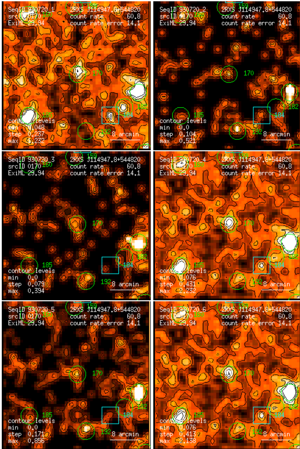
Figure 170: RASS 930720: detection 0170: band rate images, Gaussian filter: (1) PSPC channels 11 – 41, (2) 52 – 90, (3) 91 – 201, (4) 11 – 235, (5) 52 – 201, (6) 11 – 201. Broad band rates in counts/ks. Band rate contour levels in counts/ks/arcmin 2 .
