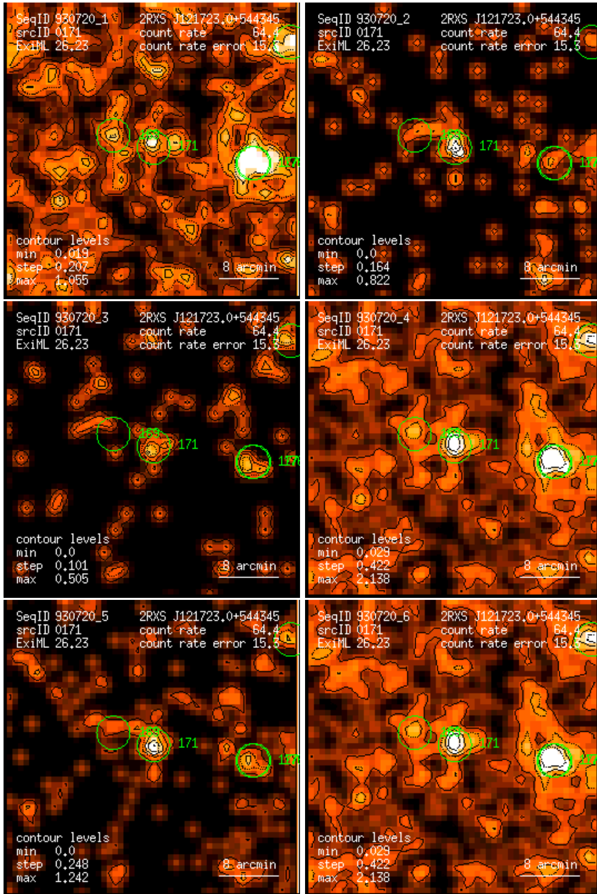
Figure 171: RASS 930720: detection 0171: band rate images, Gaussian filter: (1) PSPC channels 11 – 41, (2) 52 – 90, (3) 91 – 201, (4) 11 – 235, (5) 52 – 201, (6) 11 – 201. Broad band rates in counts/ks. Band rate contour levels in counts/ks/arcmin 2 .
