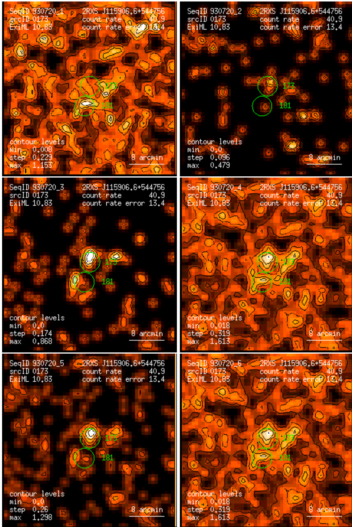
Figure 173: RASS 930720: detection 0173: band rate images, Gaussian filter: (1) PSPC channels 11 – 41, (2) 52 – 90, (3) 91 – 201, (4) 11 – 235, (5) 52 – 201, (6) 11 – 201. Broad band rates in counts/ks. Band rate contour levels in counts/ks/arcmin 2 .
