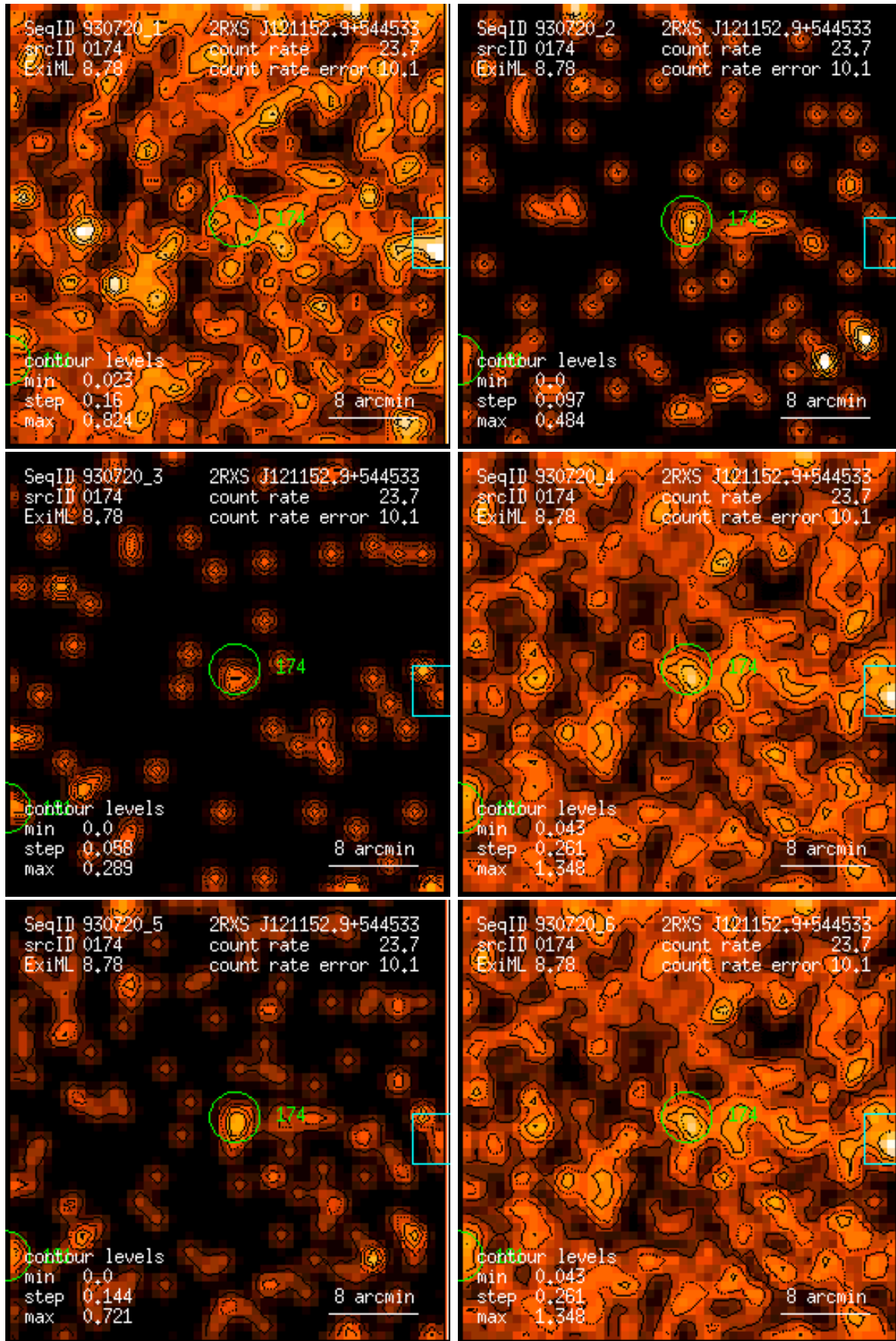
Figure 174: RASS 930720: detection 0174: band rate images, Gaussian filter: (1) PSPC channels 11 – 41, (2) 52 – 90, (3) 91 – 201, (4) 11 – 235, (5) 52 – 201, (6) 11 – 201. Broad band rates in counts/ks. Band rate contour levels in counts/ks/arcmin 2 .
