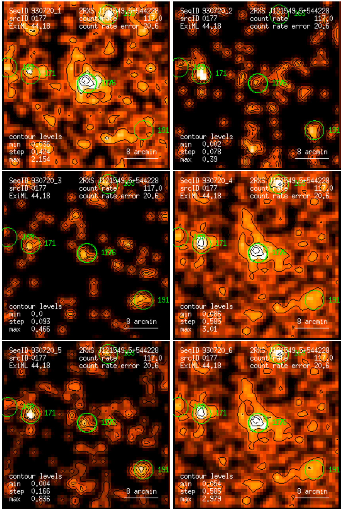
Figure 177: RASS 930720: detection 0177: band rate images, Gaussian filter: (1) PSPC channels 11 – 41, (2) 52 – 90, (3) 91 – 201, (4) 11 – 235, (5) 52 – 201, (6) 11 – 201. Broad band rates in counts/ks. Band rate contour levels in counts/ks/arcmin 2 .
