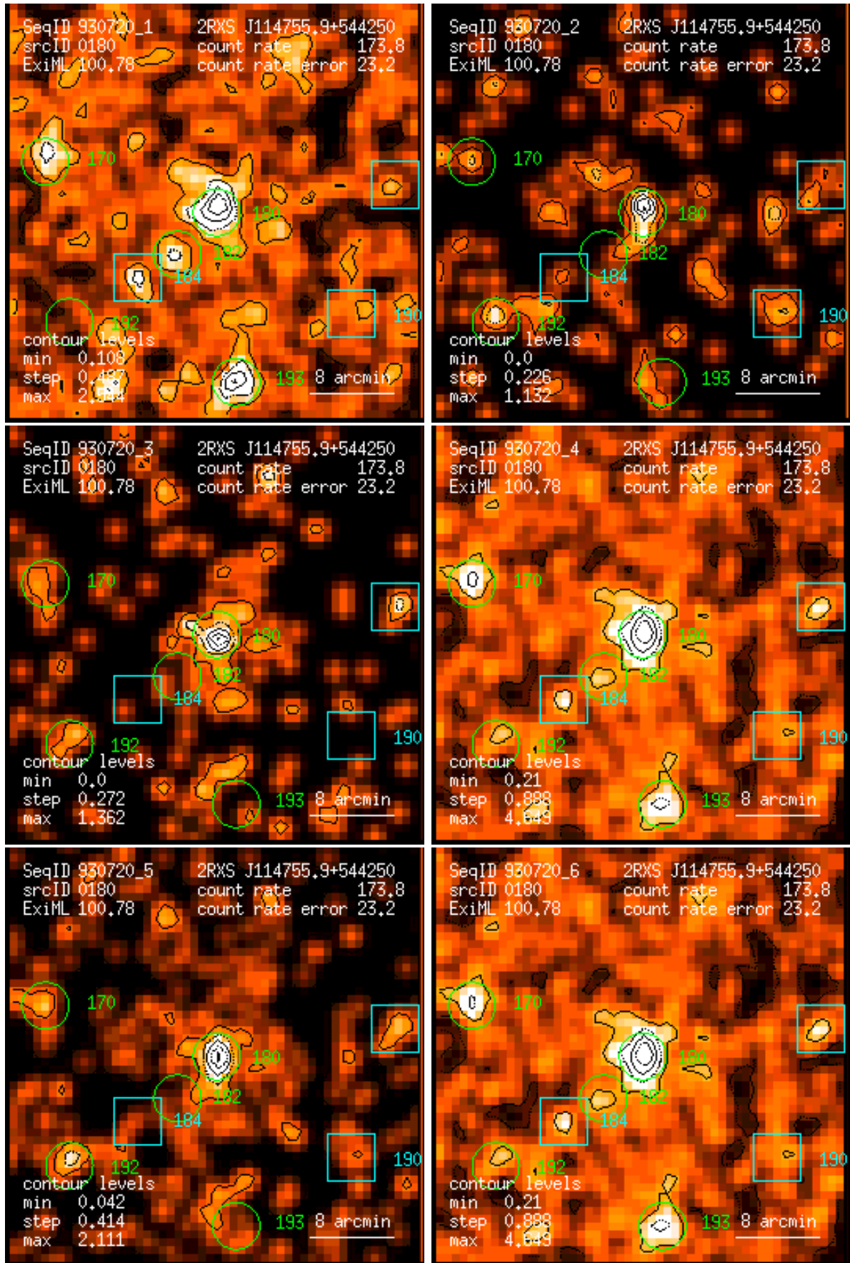
Figure 180: RASS 930720: detection 0180: band rate images, Gaussian filter: (1) PSPC channels 11 – 41, (2) 52 – 90, (3) 91 – 201, (4) 11 – 235, (5) 52 – 201, (6) 11 – 201. Broad band rates in counts/ks. Band rate contour levels in counts/ks/arcmin 2 .
