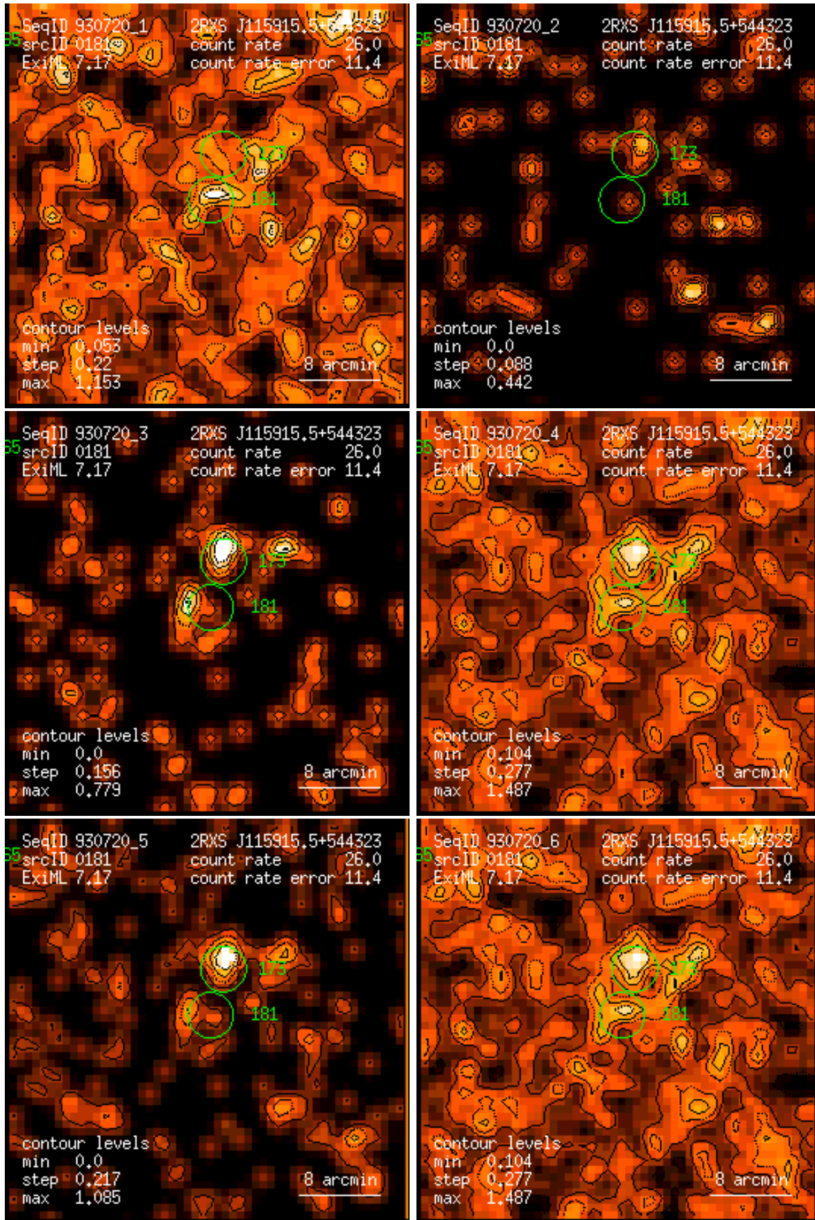
Figure 181: RASS 930720: detection 0181: band rate images, Gaussian filter: (1) PSPC channels 11 – 41, (2) 52 – 90, (3) 91 – 201, (4) 11 – 235, (5) 52 – 201, (6) 11 – 201. Broad band rates in counts/ks. Band rate contour levels in counts/ks/arcmin 2 .
