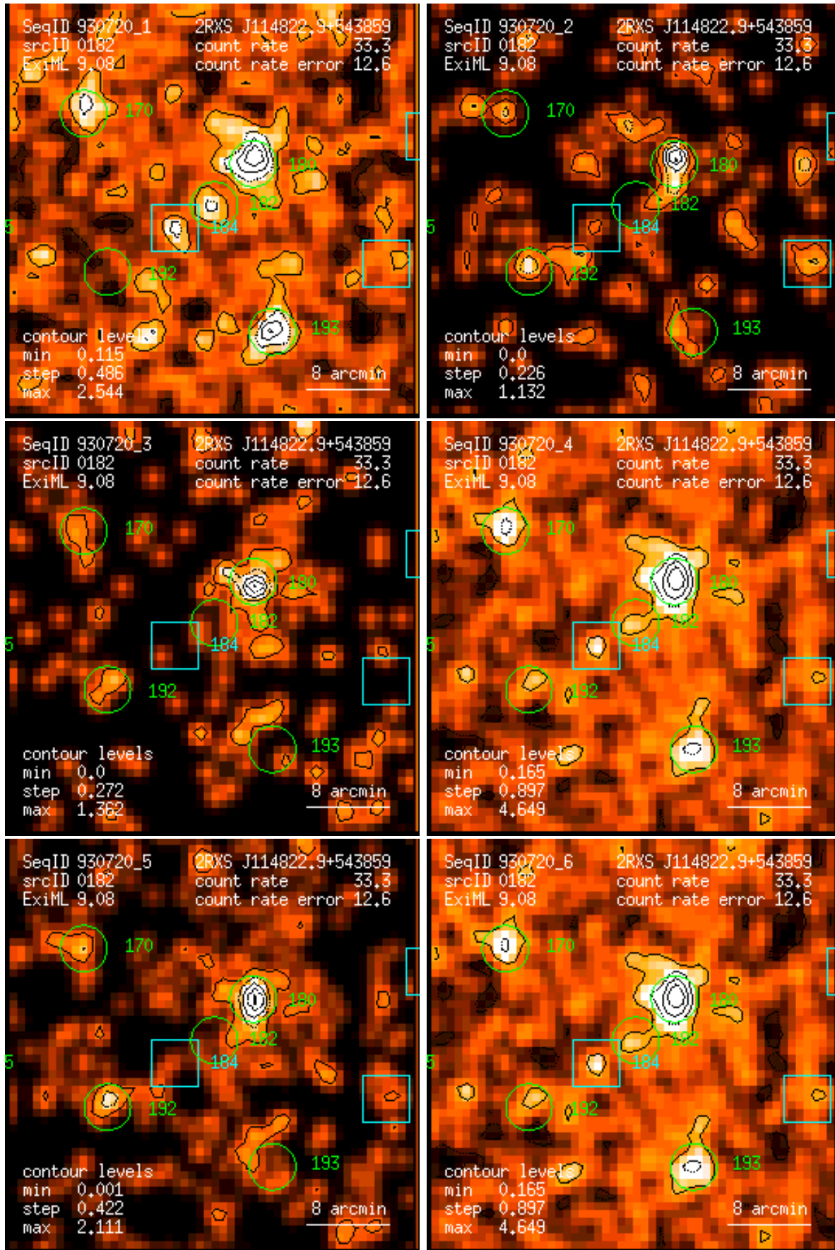
Figure 182: RASS 930720: detection 0182: band rate images, Gaussian filter: (1) PSPC channels 11 – 41, (2) 52 – 90, (3) 91 – 201, (4) 11 – 235, (5) 52 – 201, (6) 11 – 201. Broad band rates in counts/ks. Band rate contour levels in counts/ks/arcmin 2 .
