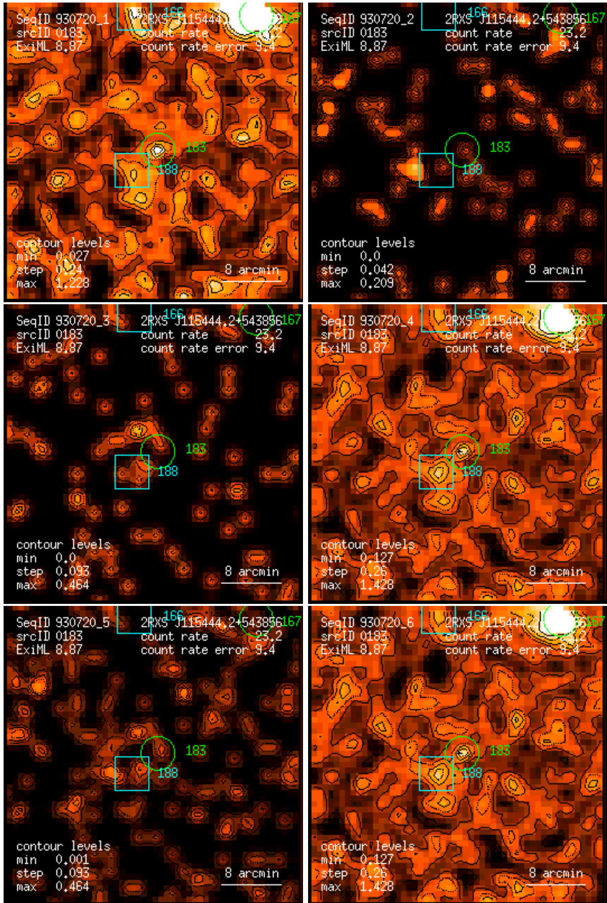
Figure 183: RASS 930720: detection 0183: band rate images, Gaussian filter: (1) PSPC channels 11 – 41, (2) 52 – 90, (3) 91 – 201, (4) 11 – 235, (5) 52 – 201, (6) 11 – 201. Broad band rates in counts/ks. Band rate contour levels in counts/ks/arcmin 2 .
