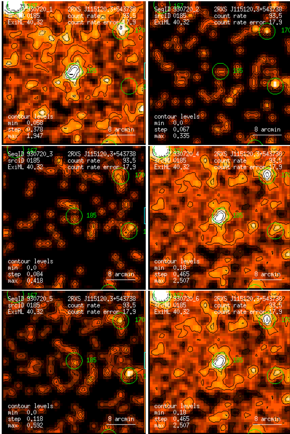
Figure 185: RASS 930720: detection 0185: band rate images, Gaussian filter: (1) PSPC channels 11 – 41, (2) 52 – 90, (3) 91 – 201, (4) 11 – 235, (5) 52 – 201, (6) 11 – 201. Broad band rates in counts/ks. Band rate contour levels in counts/ks/arcmin 2 .
