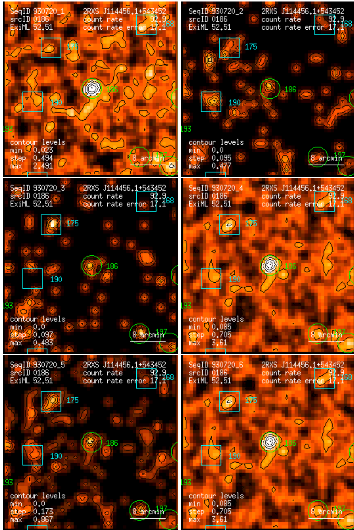
Figure 186: RASS 930720: detection 0186: band rate images, Gaussian filter: (1) PSPC channels 11 – 41, (2) 52 – 90, (3) 91 – 201, (4) 11 – 235, (5) 52 – 201, (6) 11 – 201. Broad band rates in counts/ks. Band rate contour levels in counts/ks/arcmin 2 .
