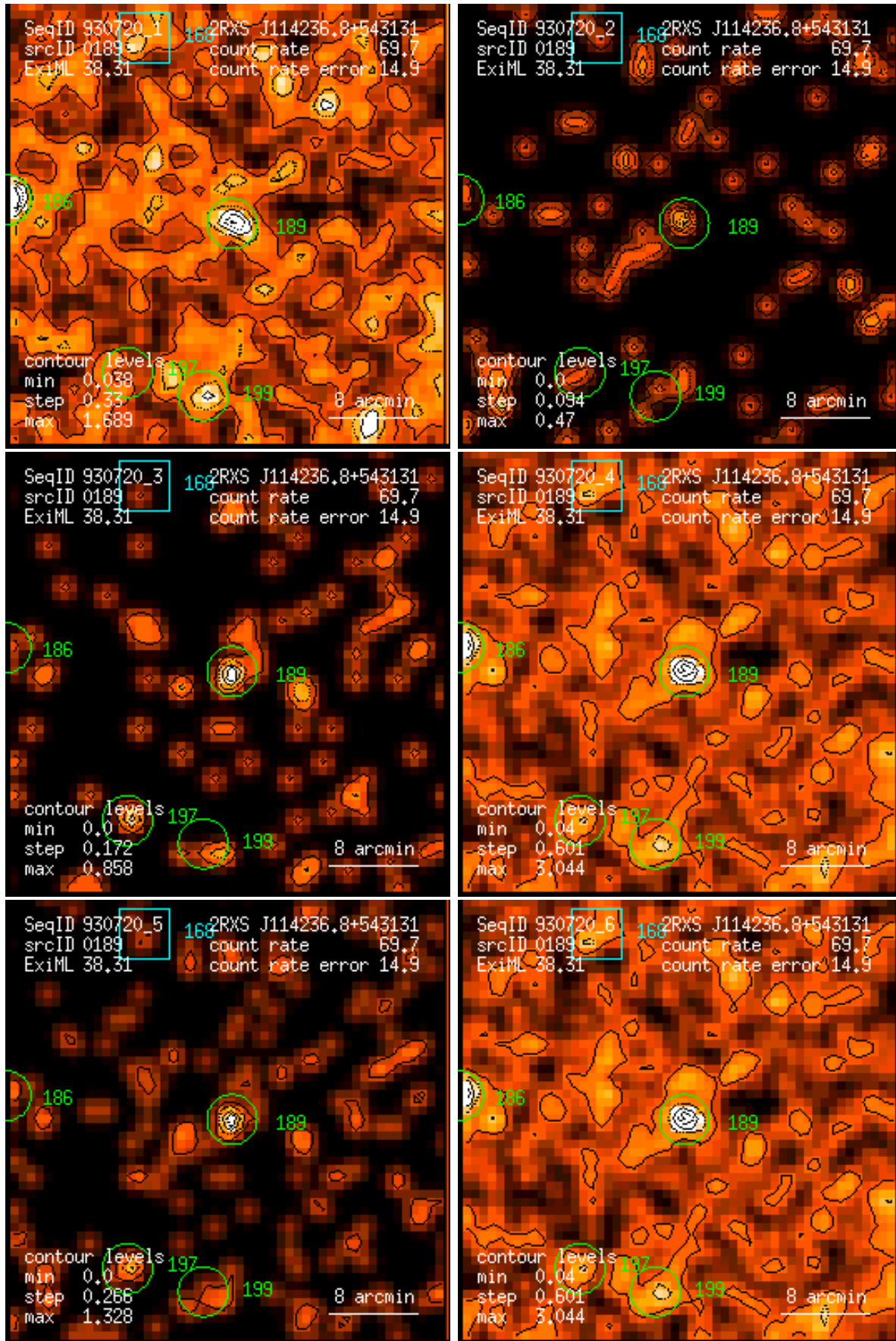
Figure 189: RASS 930720: detection 0189: band rate images, Gaussian filter: (1) PSPC channels 11 – 41, (2) 52 – 90, (3) 91 – 201, (4) 11 – 235, (5) 52 – 201, (6) 11 – 201. Broad band rates in counts/ks. Band rate contour levels in counts/ks/arcmin 2 .
