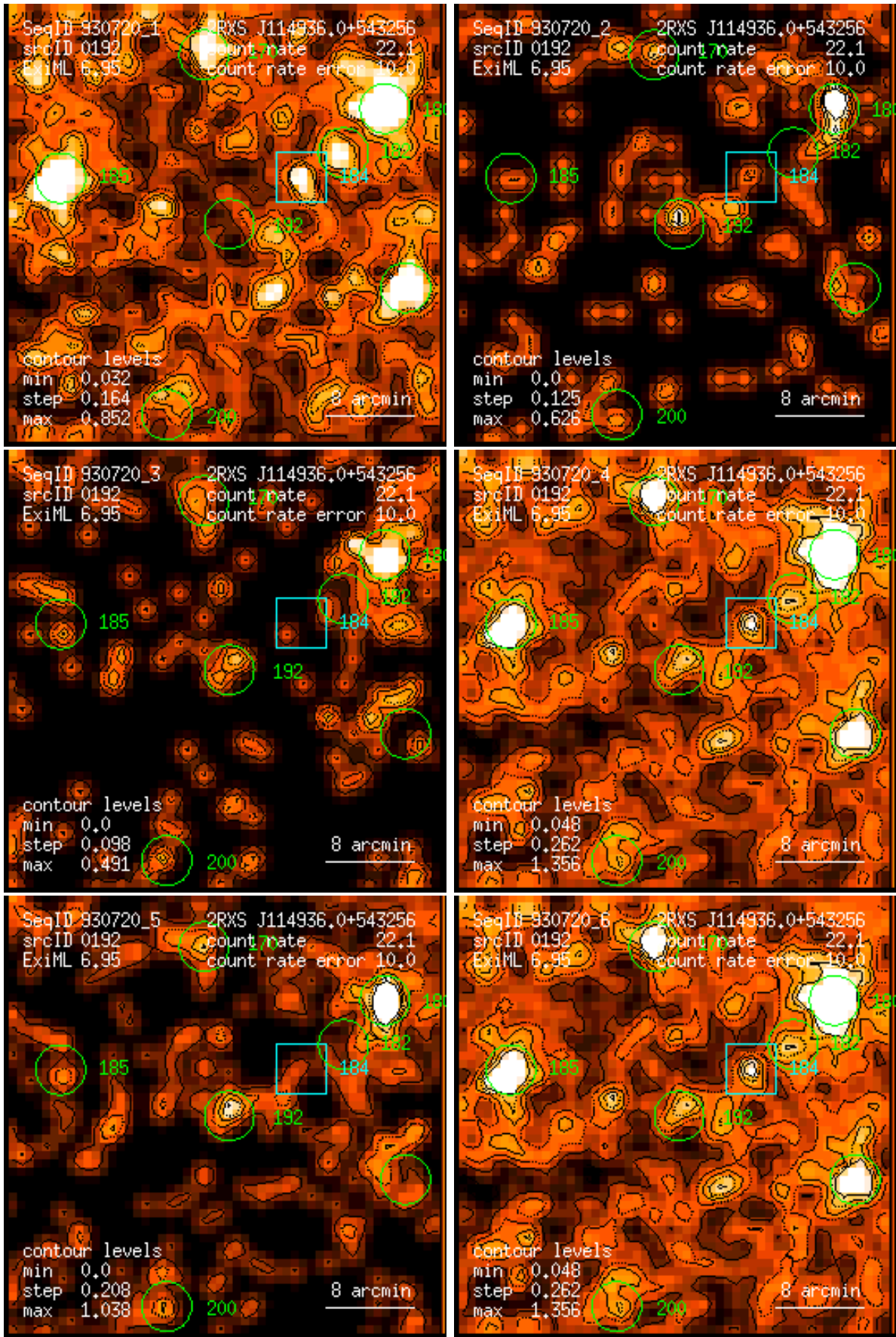
Figure 192: RASS 930720: detection 0192: band rate images, Gaussian filter: (1) PSPC channels 11 – 41, (2) 52 – 90, (3) 91 – 201, (4) 11 – 235, (5) 52 – 201, (6) 11 – 201. Broad band rates in counts/ks. Band rate contour levels in counts/ks/arcmin 2 .
