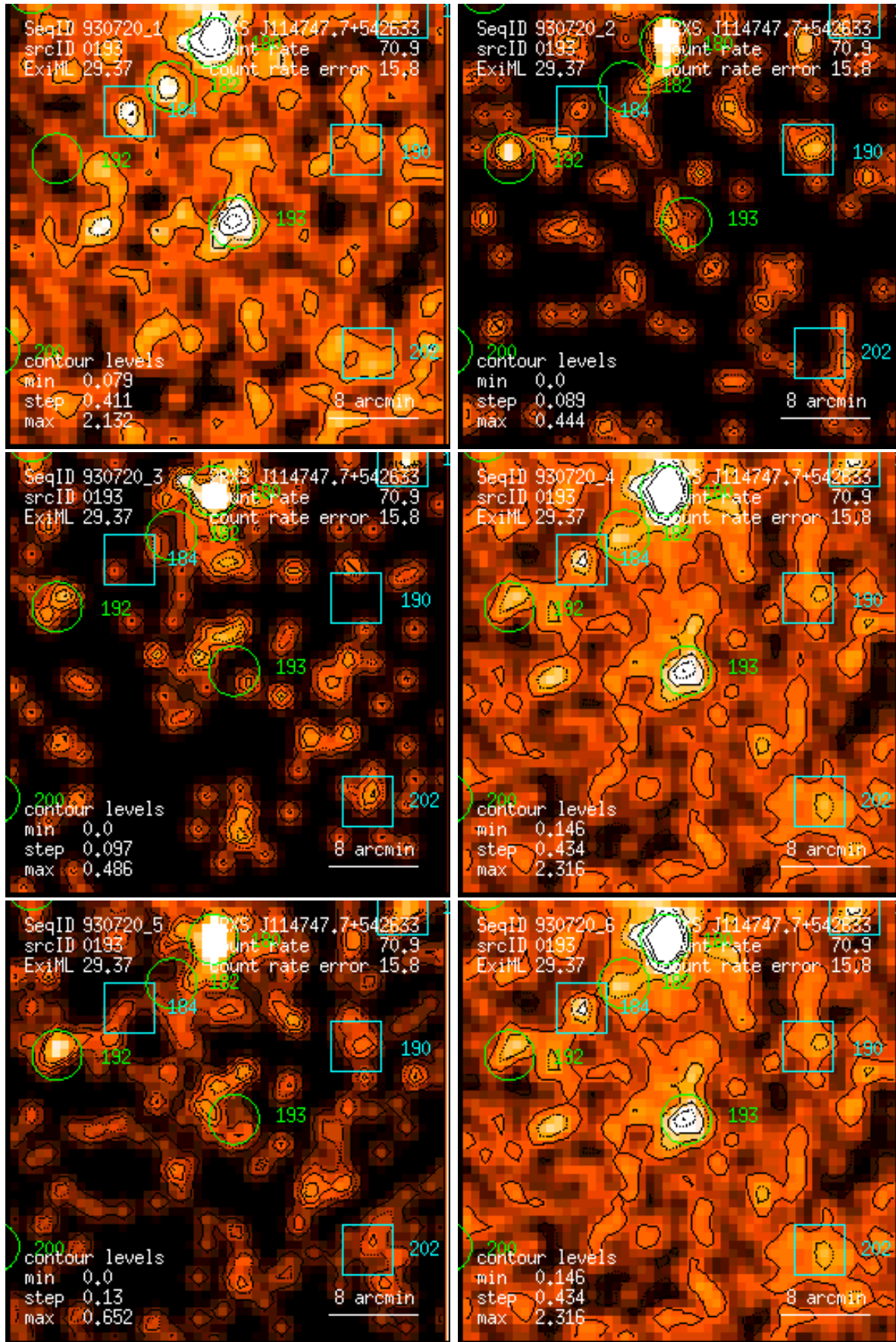
Figure 193: RASS 930720: detection 0193: band rate images, Gaussian filter: (1) PSPC channels 11 – 41, (2) 52 – 90, (3) 91 – 201, (4) 11 – 235, (5) 52 – 201, (6) 11 – 201. Broad band rates in counts/ks. Band rate contour levels in counts/ks/arcmin 2 .
