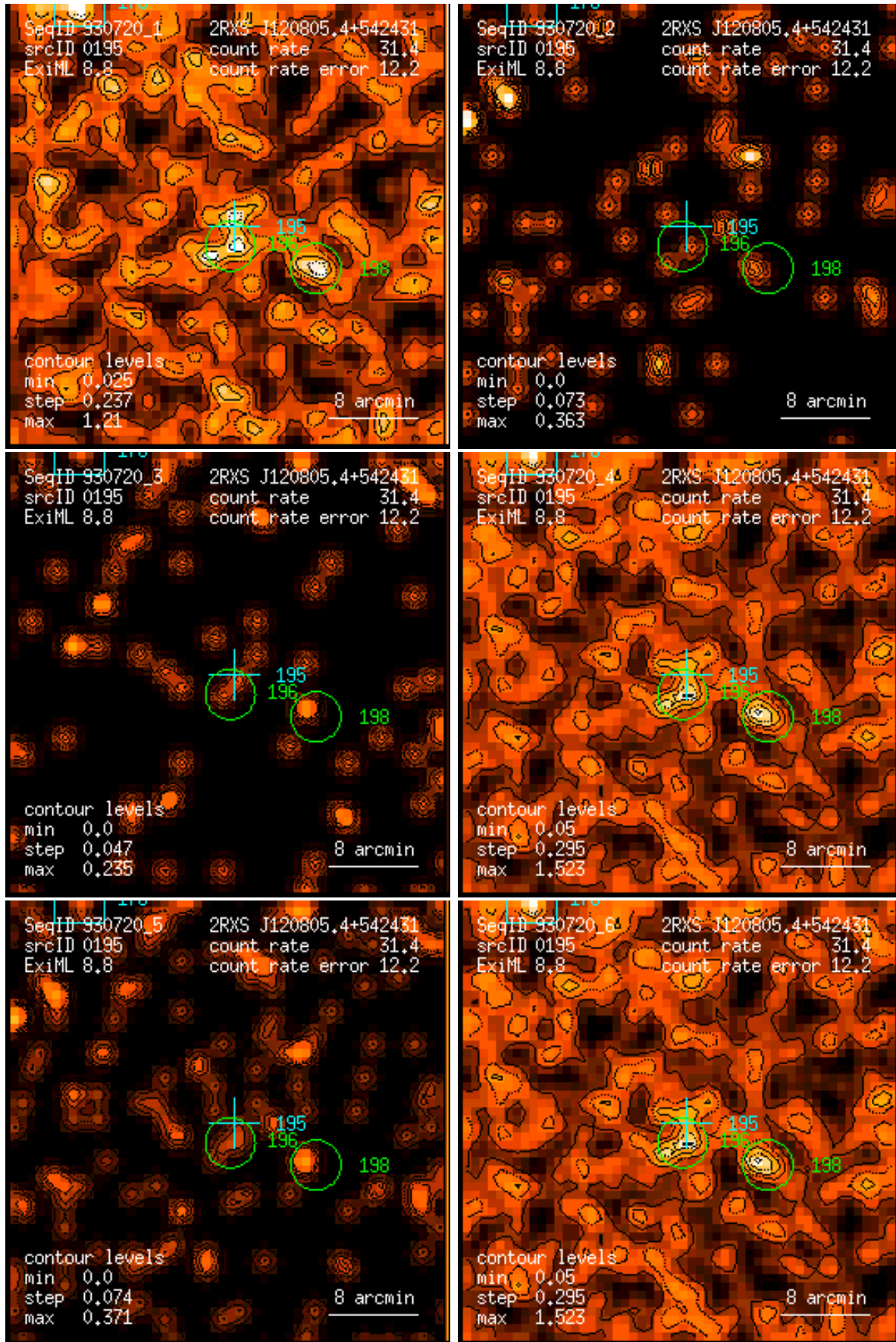
Figure 195: RASS 930720: detection 0195: band rate images, Gaussian filter: (1) PSPC channels 11 – 41, (2) 52 – 90, (3) 91 – 201, (4) 11 – 235, (5) 52 – 201, (6) 11 – 201. Broad band rates in counts/ks. Band rate contour levels in counts/ks/arcmin 2 .
