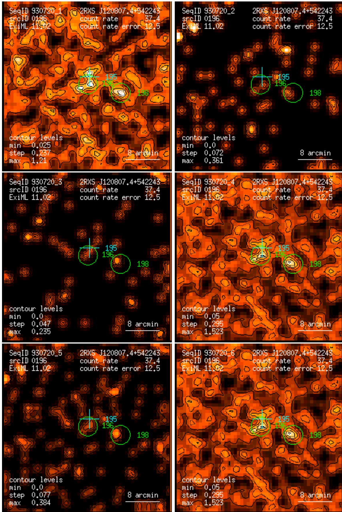
Figure 196: RASS 930720: detection 0196: band rate images, Gaussian filter: (1) PSPC channels 11 – 41, (2) 52 – 90, (3) 91 – 201, (4) 11 – 235, (5) 52 – 201, (6) 11 – 201. Broad band rates in counts/ks. Band rate contour levels in counts/ks/arcmin 2 .
