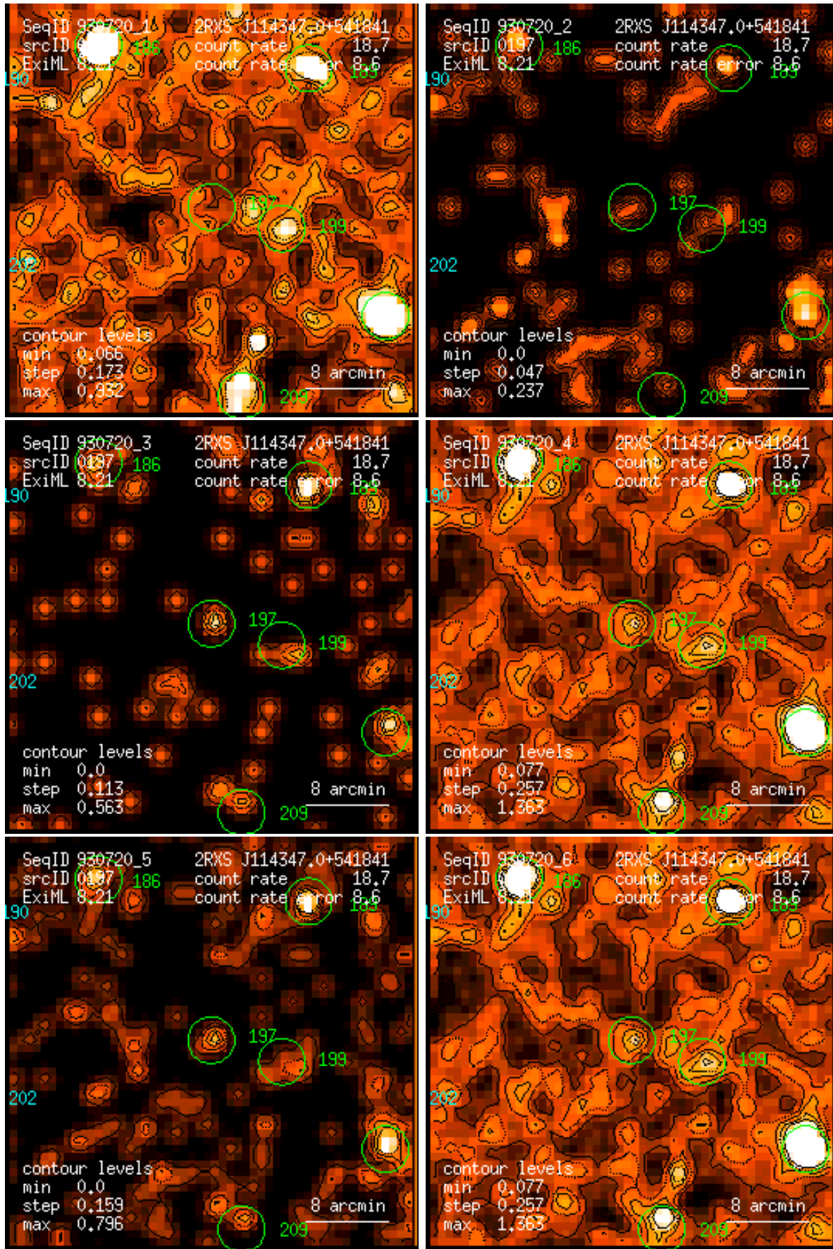
Figure 197: RASS 930720: detection 0197: band rate images, Gaussian filter: (1) PSPC channels 11 – 41, (2) 52 – 90, (3) 91 – 201, (4) 11 – 235, (5) 52 – 201, (6) 11 – 201. Broad band rates in counts/ks. Band rate contour levels in counts/ks/arcmin 2 .
