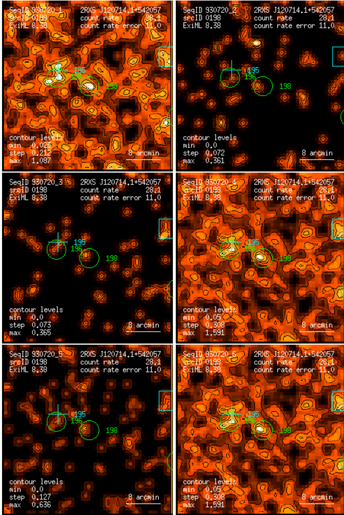
Figure 198: RASS 930720: detection 0198: band rate images, Gaussian filter: (1) PSPC channels 11 – 41, (2) 52 – 90, (3) 91 – 201, (4) 11 – 235, (5) 52 – 201, (6) 11 – 201. Broad band rates in counts/ks. Band rate contour levels in counts/ks/arcmin 2 .
