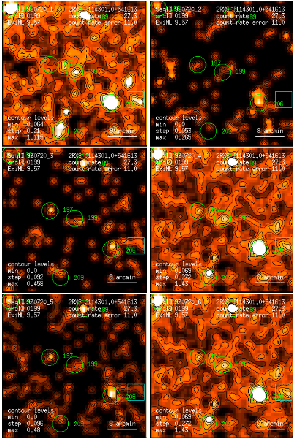
Figure 199: RASS 930720: detection 0199: band rate images, Gaussian filter: (1) PSPC channels 11 – 41, (2) 52 – 90, (3) 91 – 201, (4) 11 – 235, (5) 52 – 201, (6) 11 – 201. Broad band rates in counts/ks. Band rate contour levels in counts/ks/arcmin 2 .
