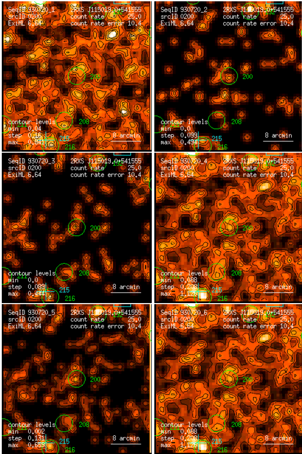
Figure 200: RASS 930720: detection 0200: band rate images, Gaussian filter: (1) PSPC channels 11 – 41, (2) 52 – 90, (3) 91 – 201, (4) 11 – 235, (5) 52 – 201, (6) 11 – 201. Broad band rates in counts/ks. Band rate contour levels in counts/ks/arcmin 2 .
