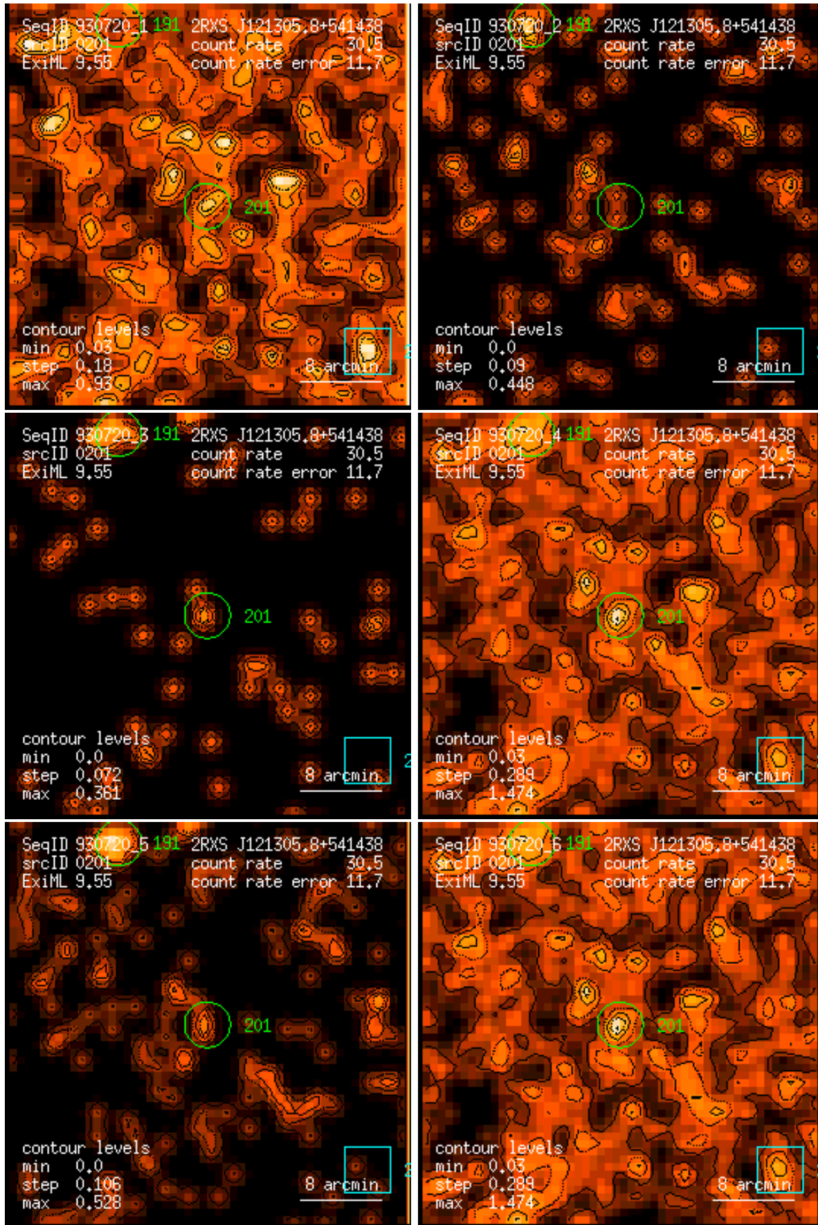
Figure 201: RASS 930720: detection 0201: band rate images, Gaussian filter: (1) PSPC channels 11 – 41, (2) 52 – 90, (3) 91 – 201, (4) 11 – 235, (5) 52 – 201, (6) 11 – 201. Broad band rates in counts/ks. Band rate contour levels in counts/ks/arcmin 2 .
