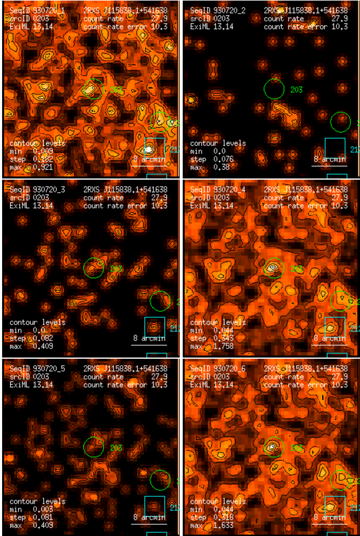
Figure 203: RASS 930720: detection 0203: band rate images, Gaussian filter: (1) PSPC channels 11 – 41, (2) 52 – 90, (3) 91 – 201, (4) 11 – 235, (5) 52 – 201, (6) 11 – 201. Broad band rates in counts/ks. Band rate contour levels in counts/ks/arcmin 2 .
