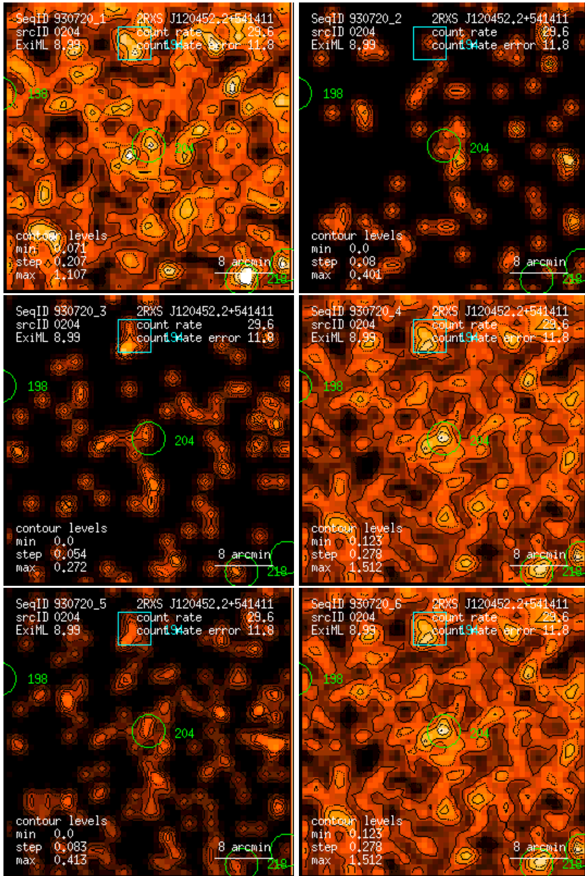
Figure 204: RASS 930720: detection 0204: band rate images, Gaussian filter: (1) PSPC channels 11 – 41, (2) 52 – 90, (3) 91 – 201, (4) 11 – 235, (5) 52 – 201, (6) 11 – 201. Broad band rates in counts/ks. Band rate contour levels in counts/ks/arcmin 2 .
