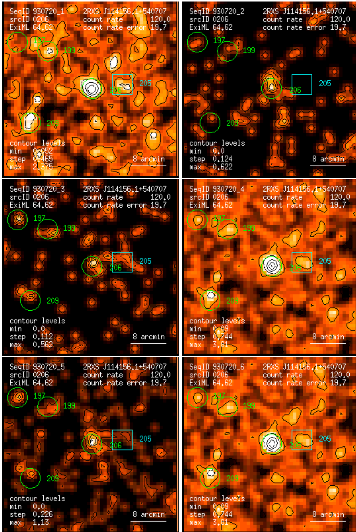
Figure 206: RASS 930720: detection 0206: band rate images, Gaussian filter: (1) PSPC channels 11 – 41, (2) 52 – 90, (3) 91 – 201, (4) 11 – 235, (5) 52 – 201, (6) 11 – 201. Broad band rates in counts/ks. Band rate contour levels in counts/ks/arcmin 2 .
