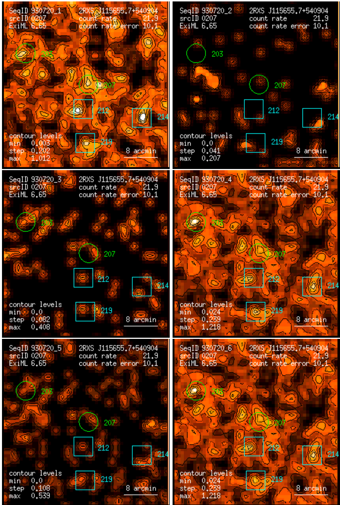
Figure 207: RASS 930720: detection 0207: band rate images, Gaussian filter: (1) PSPC channels 11 – 41, (2) 52 – 90, (3) 91 – 201, (4) 11 – 235, (5) 52 – 201, (6) 11 – 201. Broad band rates in counts/ks. Band rate contour levels in counts/ks/arcmin 2 .
