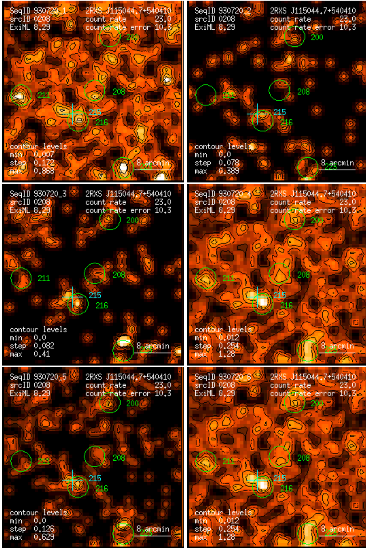
Figure 208: RASS 930720: detection 0208: band rate images, Gaussian filter: (1) PSPC channels 11 – 41, (2) 52 – 90, (3) 91 – 201, (4) 11 – 235, (5) 52 – 201, (6) 11 – 201. Broad band rates in counts/ks. Band rate contour levels in counts/ks/arcmin 2 .
